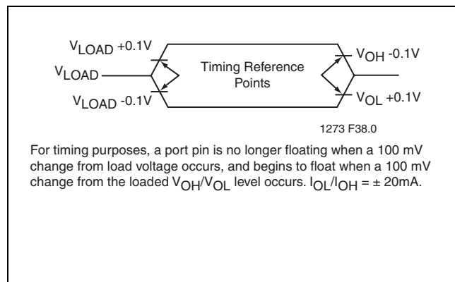
FIGURE 14-9: Float Waveform
