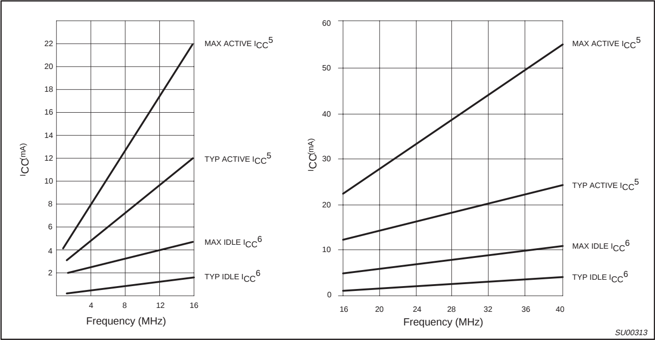
Figure 3. I_{CC} vs. Frequency Maximum I_{CC} values taken at V_{CC} max and worst case temperature. Typical I_{CC} values taken at V_{CC} = 5.0V and 25^{\circ}C . Notes 5 and 6 refer to DC Electrical Characteristics.
