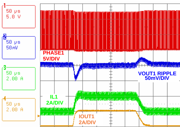
FIGURE 34. LOAD TRANSIENT
