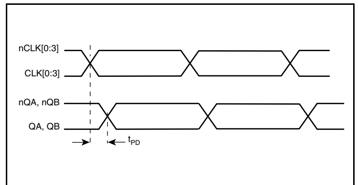
Propagation Delay
