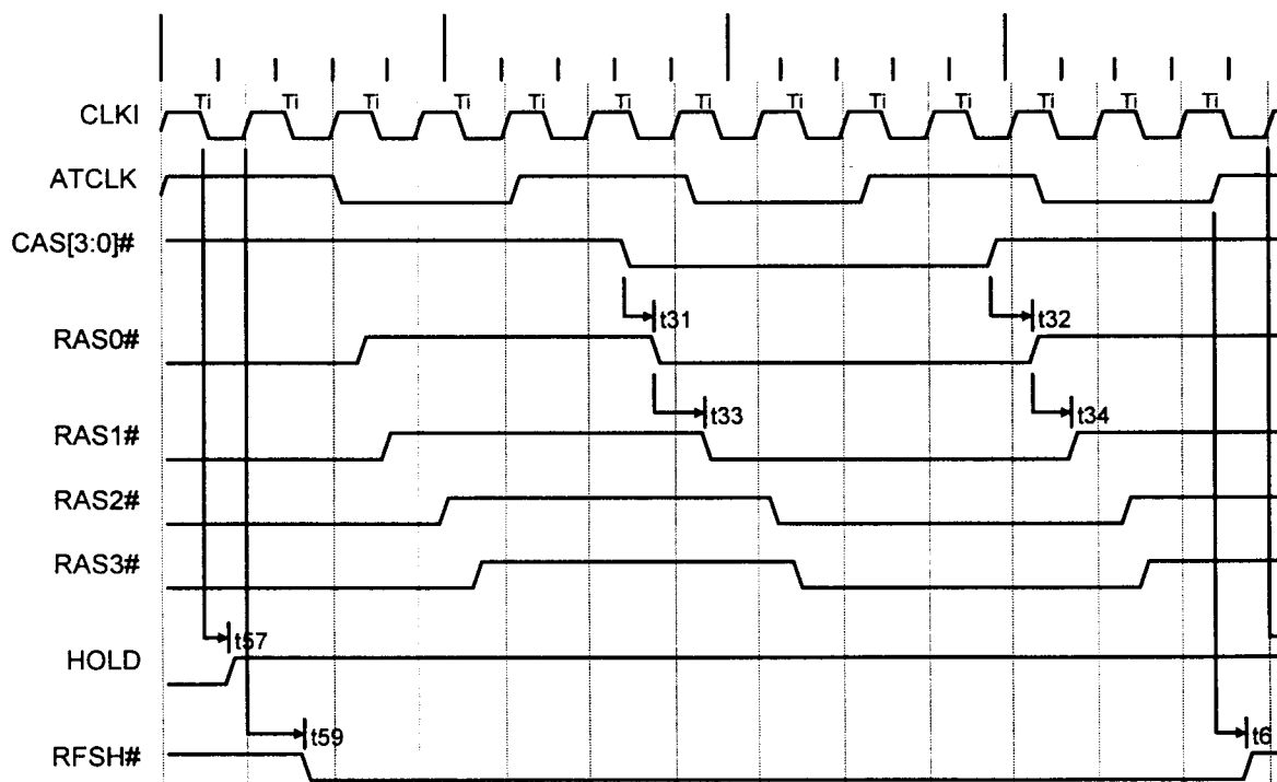
Figure 6-16 Refresh Cycle
