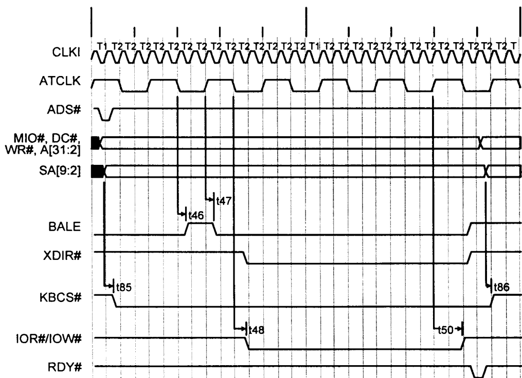
Figure 6-23 Keyboard Controller Access Cycle
