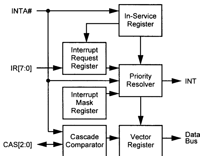
Figure 4-6 Interrupt Controller Block Diagram
