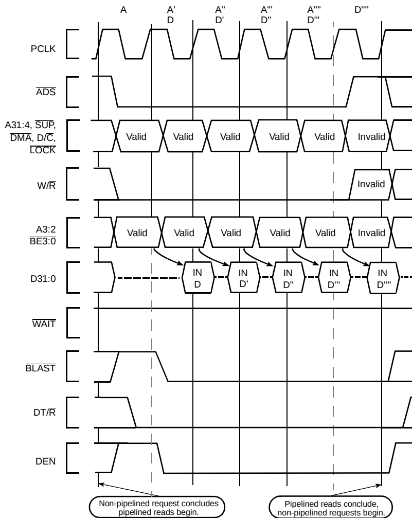
Figure 34. Non-Burst, Pipelined Read Request Without Wait States, 32-Bit Bus
