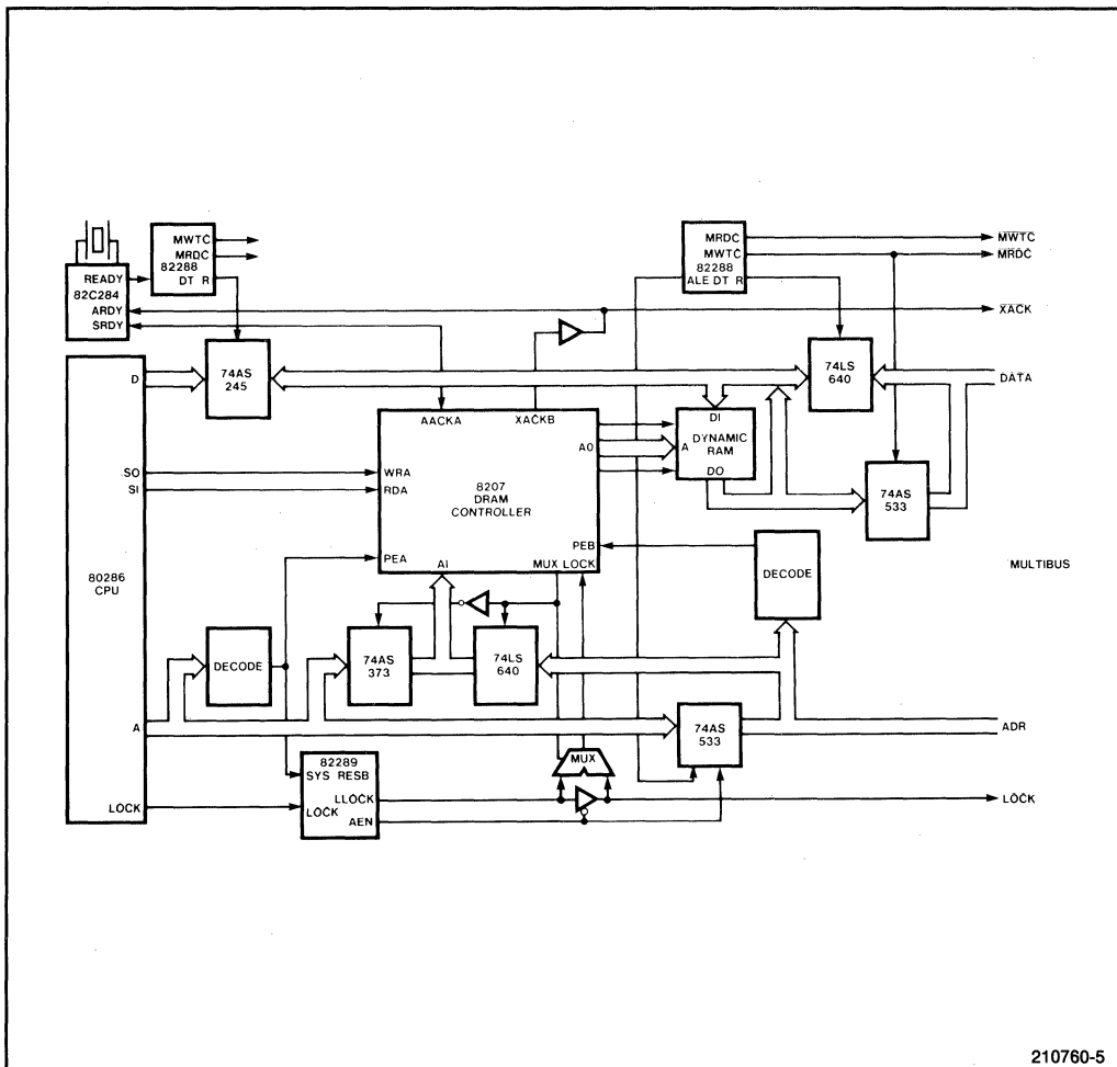
Figure 2-7. 8207 Dual-Port Subsystem
