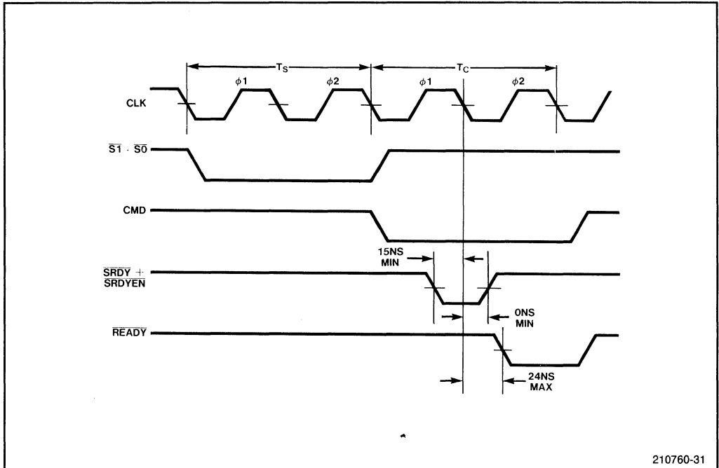
Figure 3-26. \overline{\text{SRDY}} and \overline{\text{READY}} Timing
