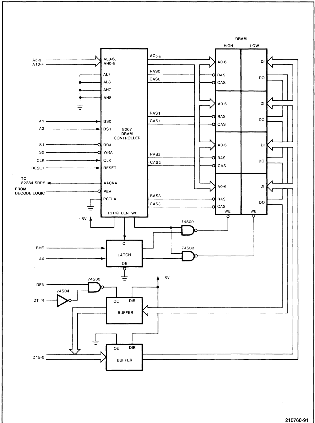
Figure 4-17. 128K-Byte Memory Subsystem
