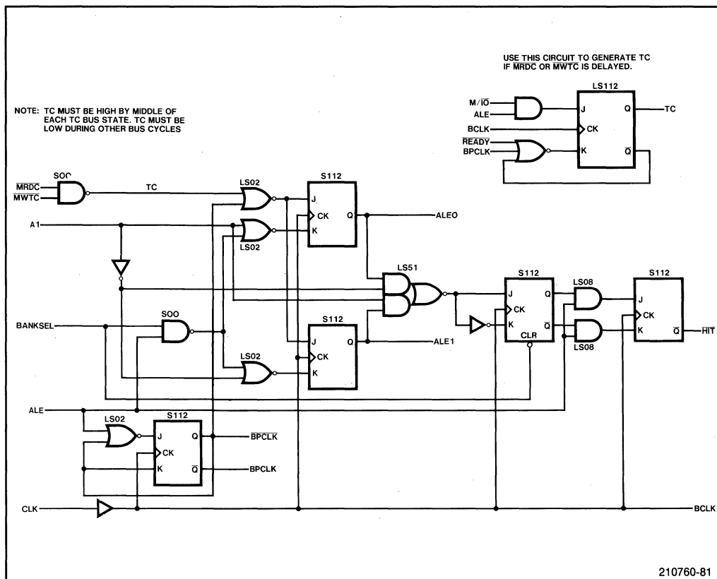
Figure 4-4. Address Strobe Generation
