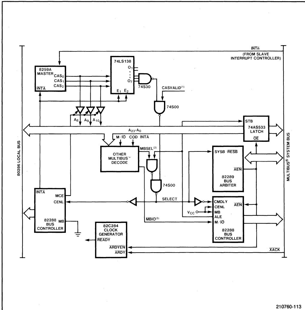
Figure 7-5. Decoding Interrupt-Acknowledge Sequences
