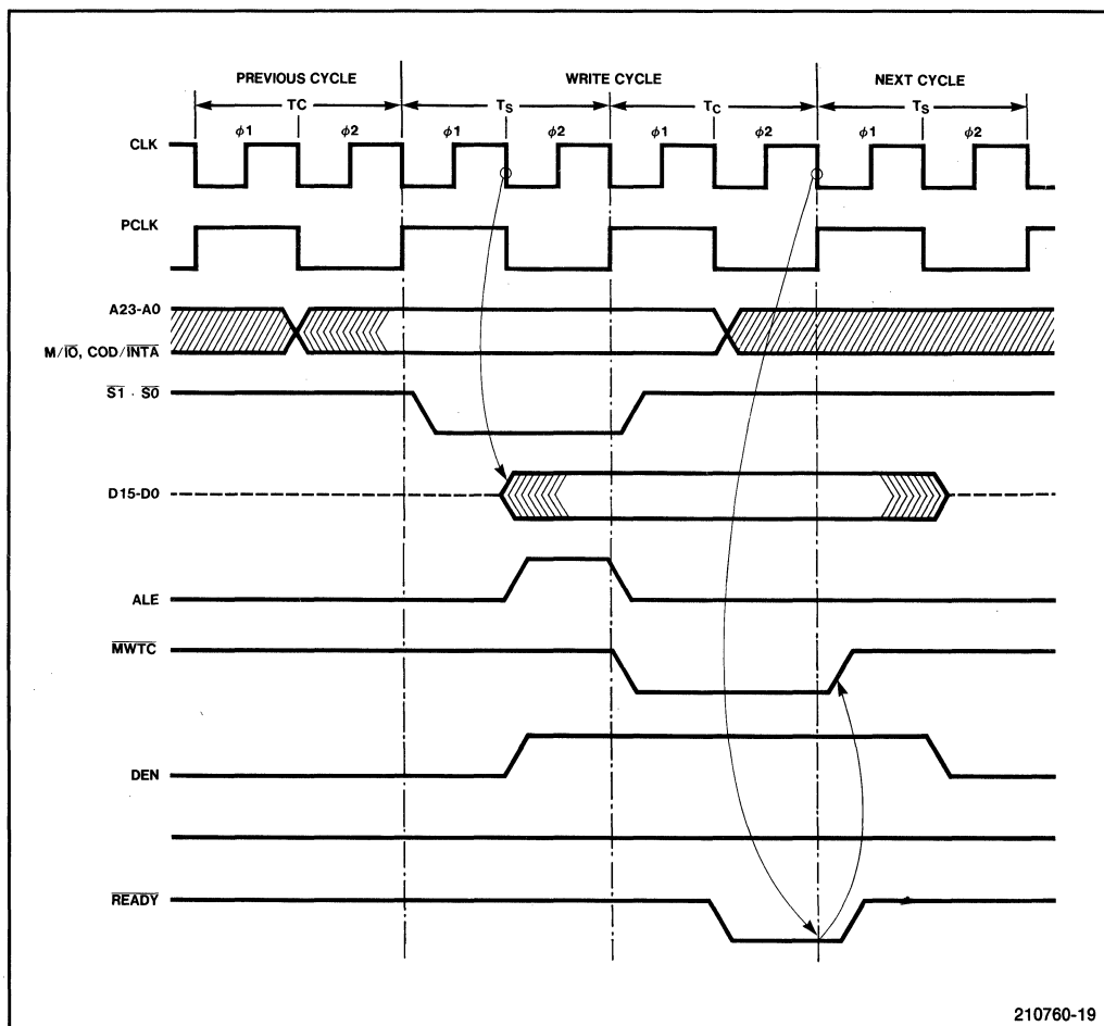
Figure 3-15. 80286 Write Cycle
