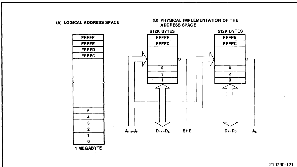
Figure 3-4. 80286 Memory Organization
