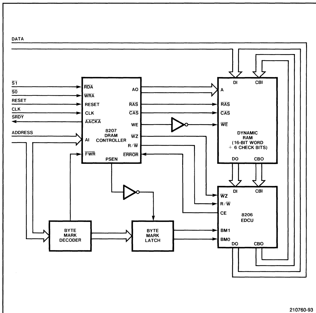
Figure 4-20. 8207 Memory Subsystem with ECC
