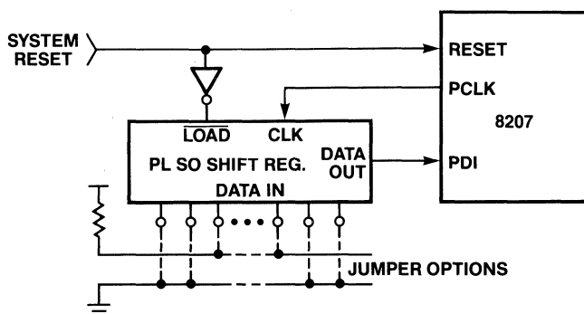
Figure 4-18. External Shift Register Interface
