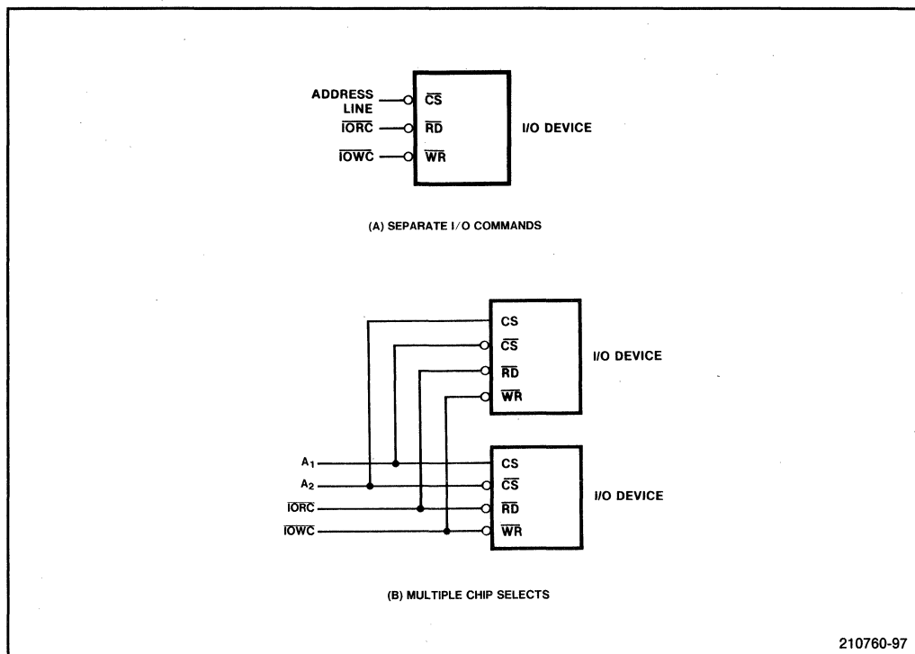
Figure 5-8. Linear Selects for I/O Devices
