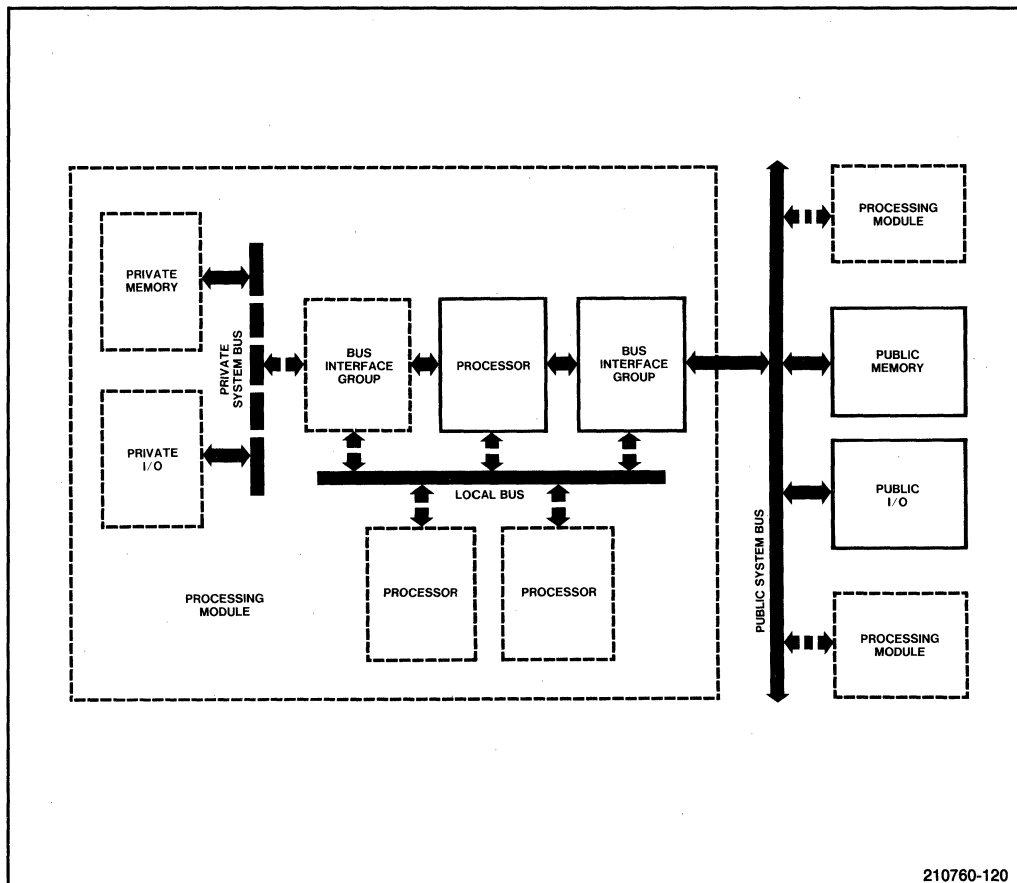
Figure 2-1. Representative 80286 System
