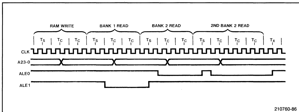
Figure 4-9. Interleaved Memory Timing
