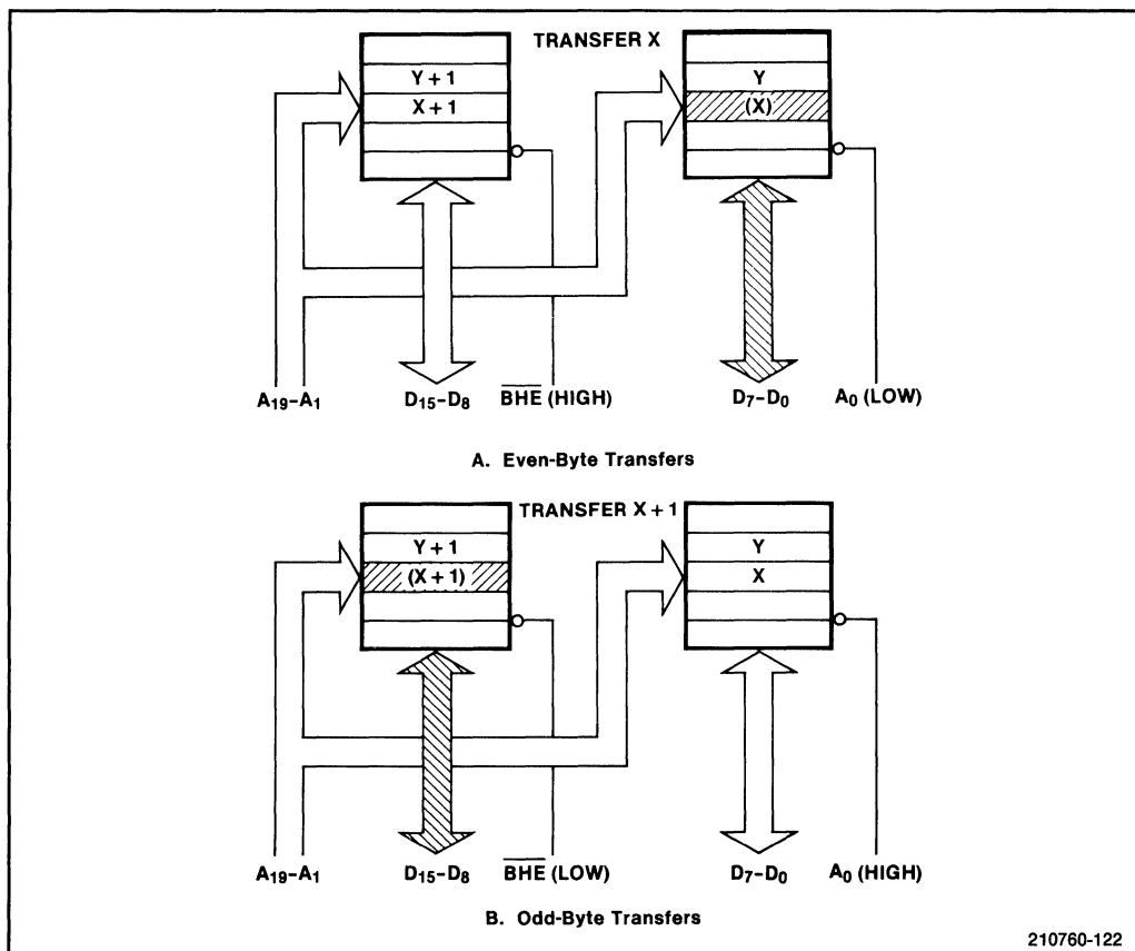
Figure 3-5. 80286 Byte Transfers
