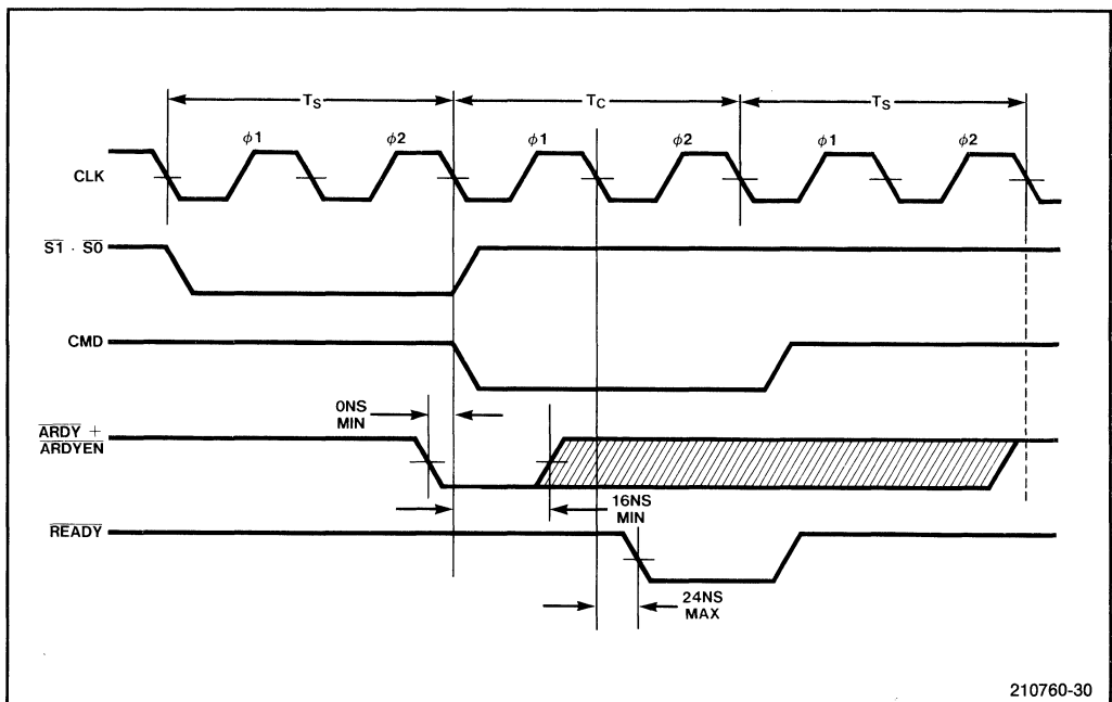
Figure 3-27. \overline{\text{ARDY}} and \overline{\text{READY}} Timing
