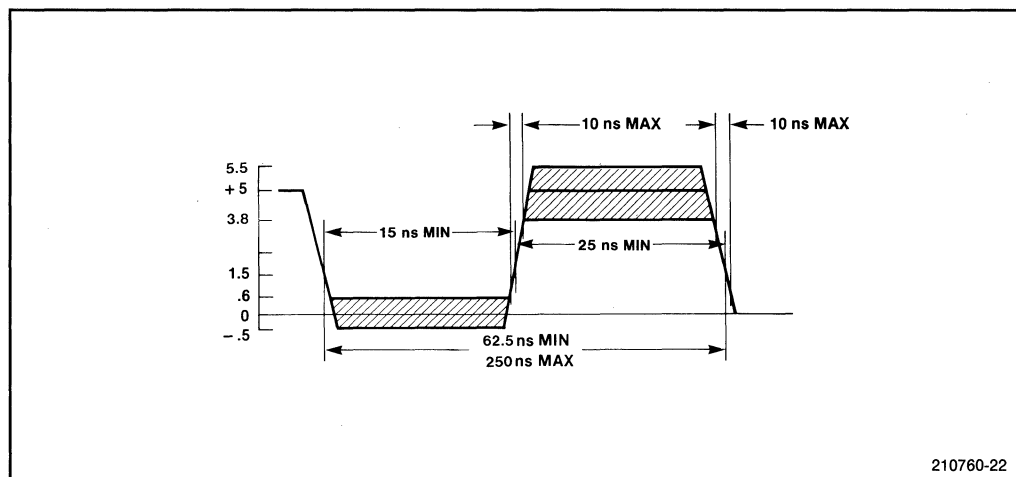
Figure 3-18. 80286 Clock Input
