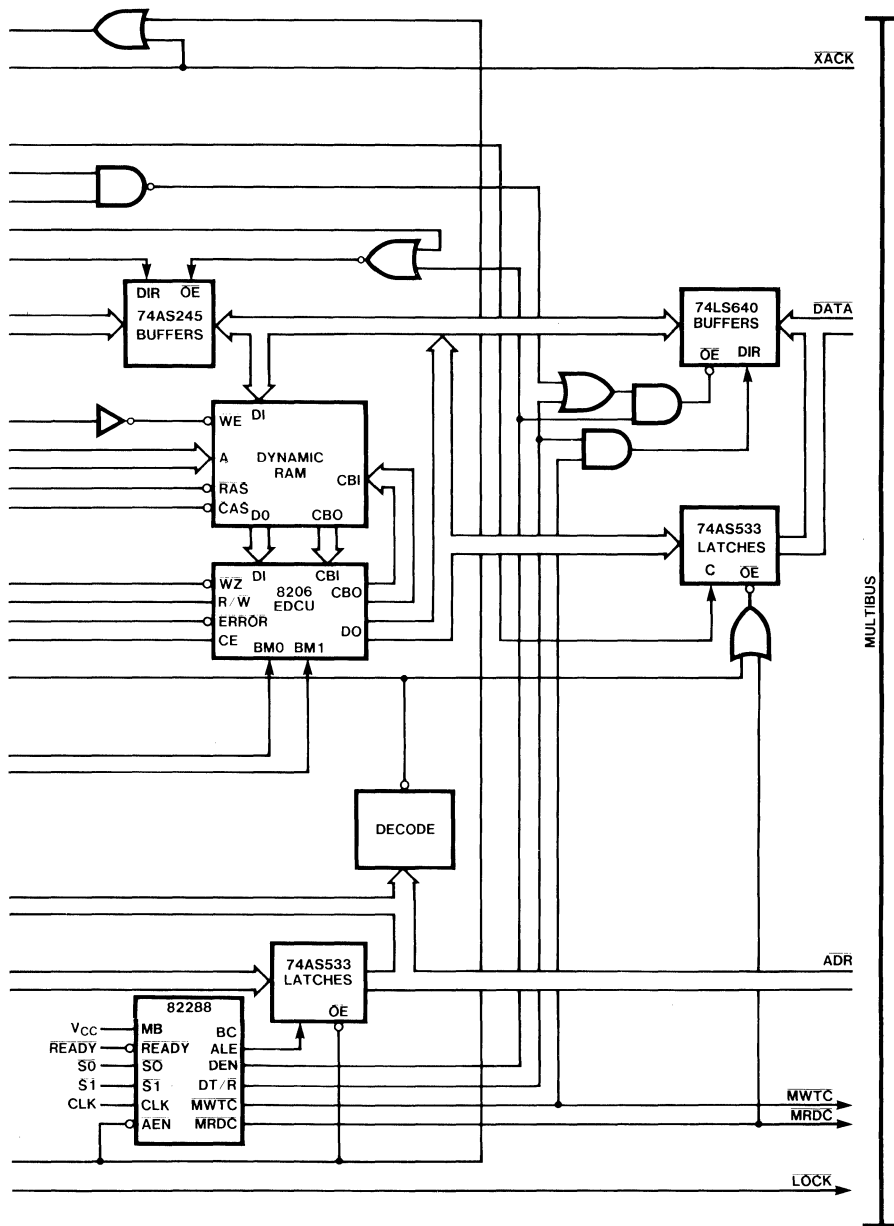
Figure 7-12. 80286 Dual-Port Memory with MULTIBUS® Interface
