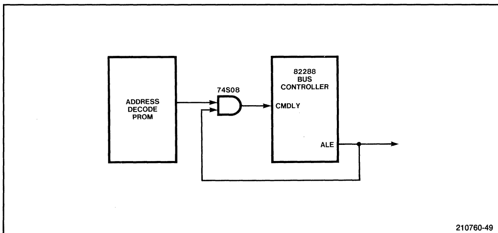
Figure 3-45. Generating \overline{CMDLY} for 0 or 1 CLK Delays
