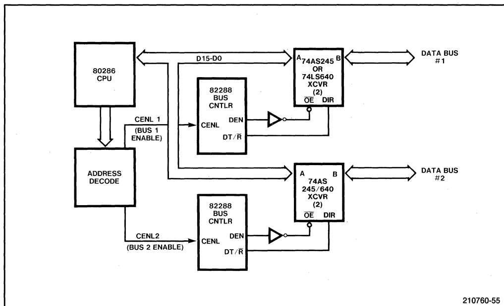
Figure 3-51. Dual Address Bus System
