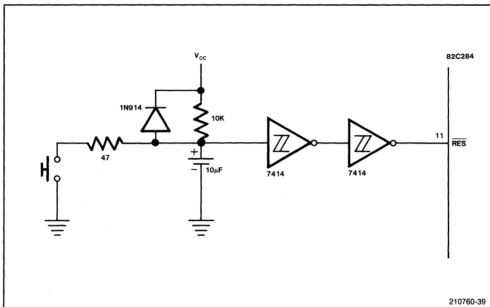
Figure 3-35. Typical RESET Timing Circuit
