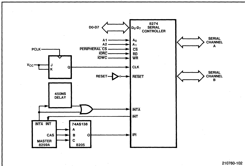
Figure 5-13. 8274 MPSC Interface
