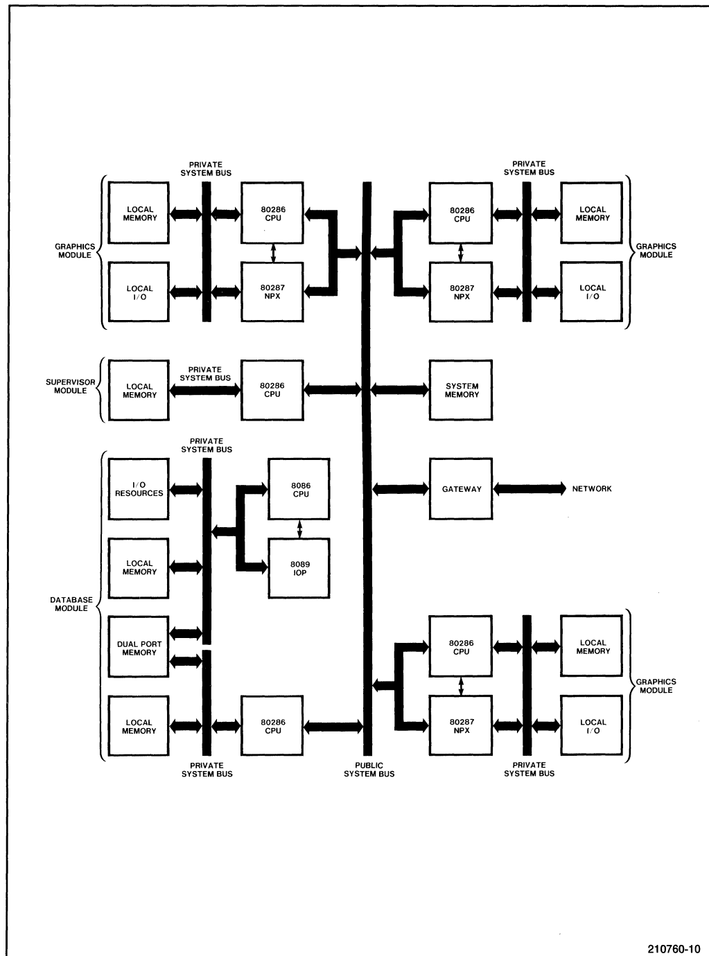
Figure 2-12. 80286 Design Example
