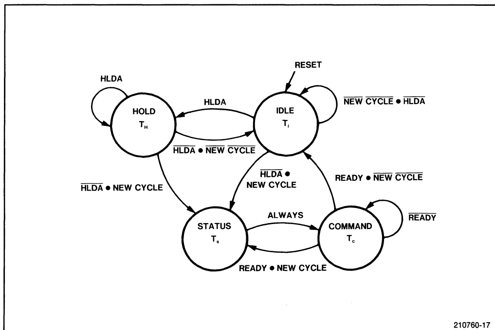
Figure 3-13. 80286 States
