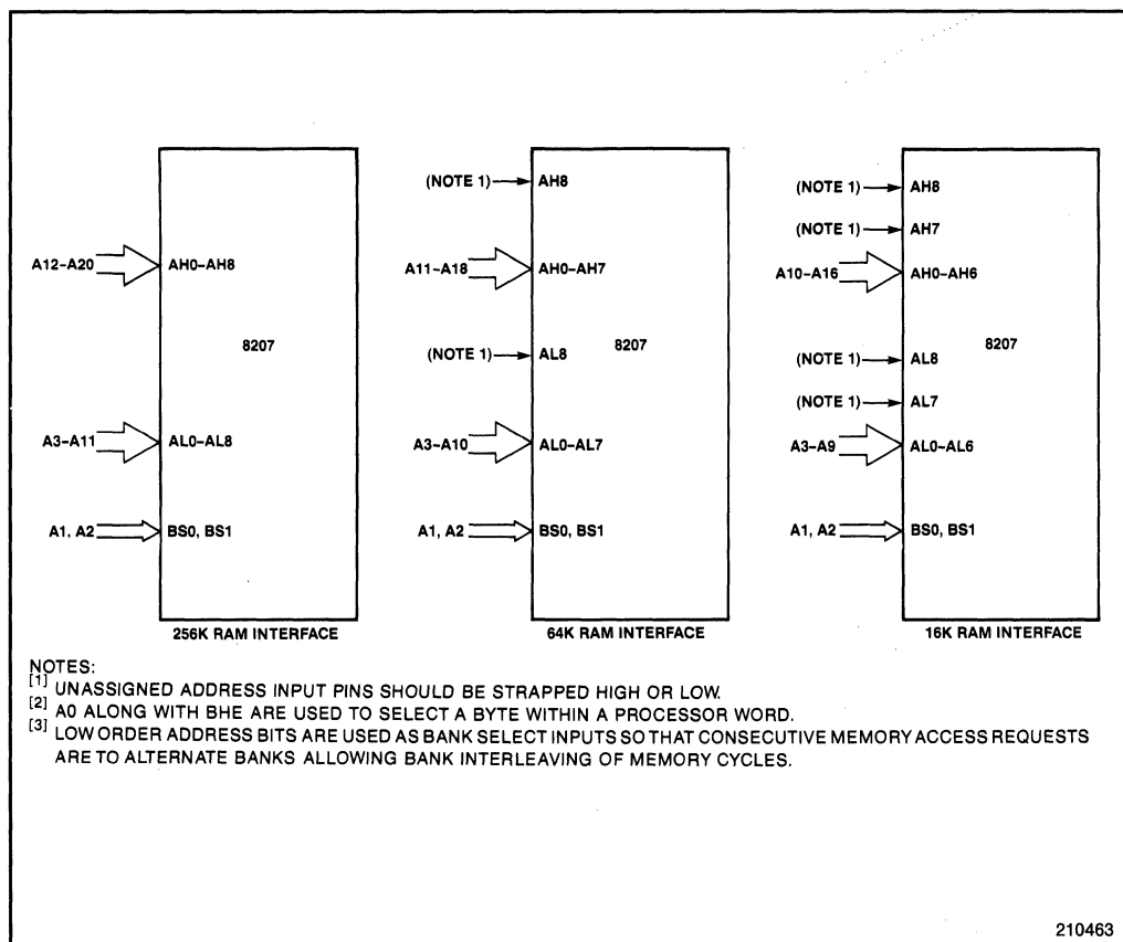
Figure 4-16. 256K, 64K, and 16K RAM Address Connections
