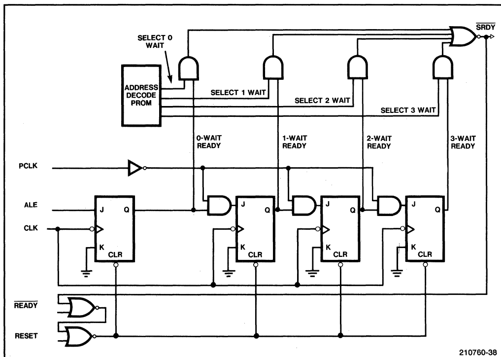
Figure 3-34. Generating from 0 to 3 Wait States
