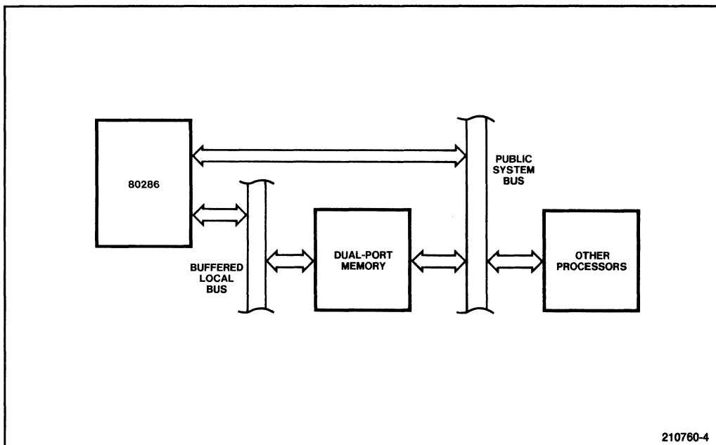
Figure 2-5. Dual-Port Memory
