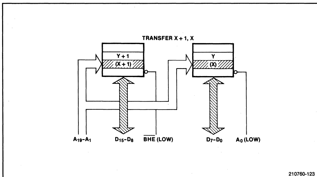
Figure 3-6. Even-Addressed Word Transfer
