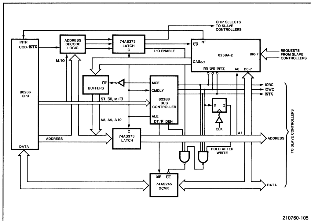
Figure 5-16. Cascaded 8259A Interrupt Controller Interface
