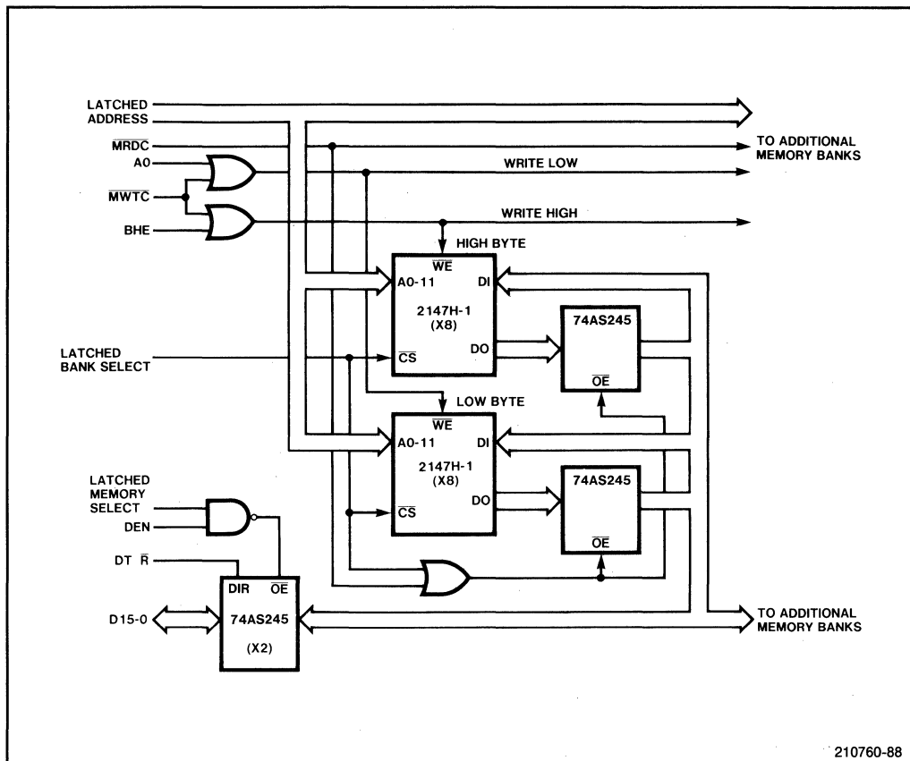
Figure 4-13. Static RAM Interface
