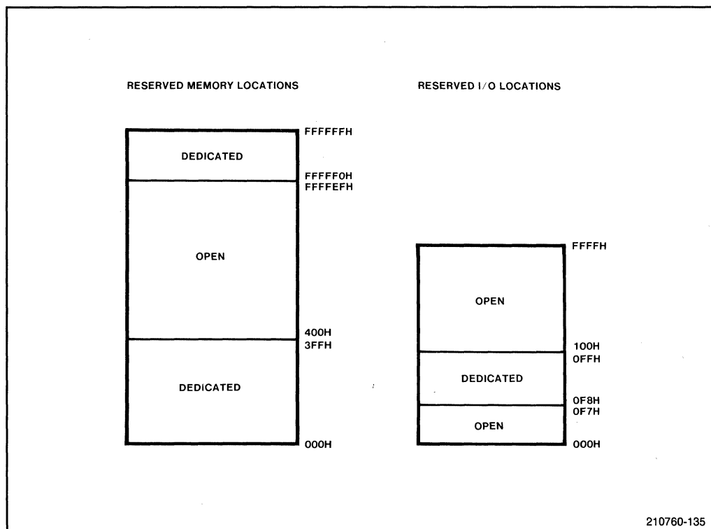
Figure 5-2. Restricted Address Regions
