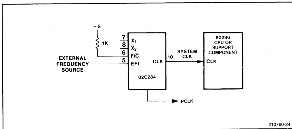
Figure 3-20. 82C284 with External Frequency Source
