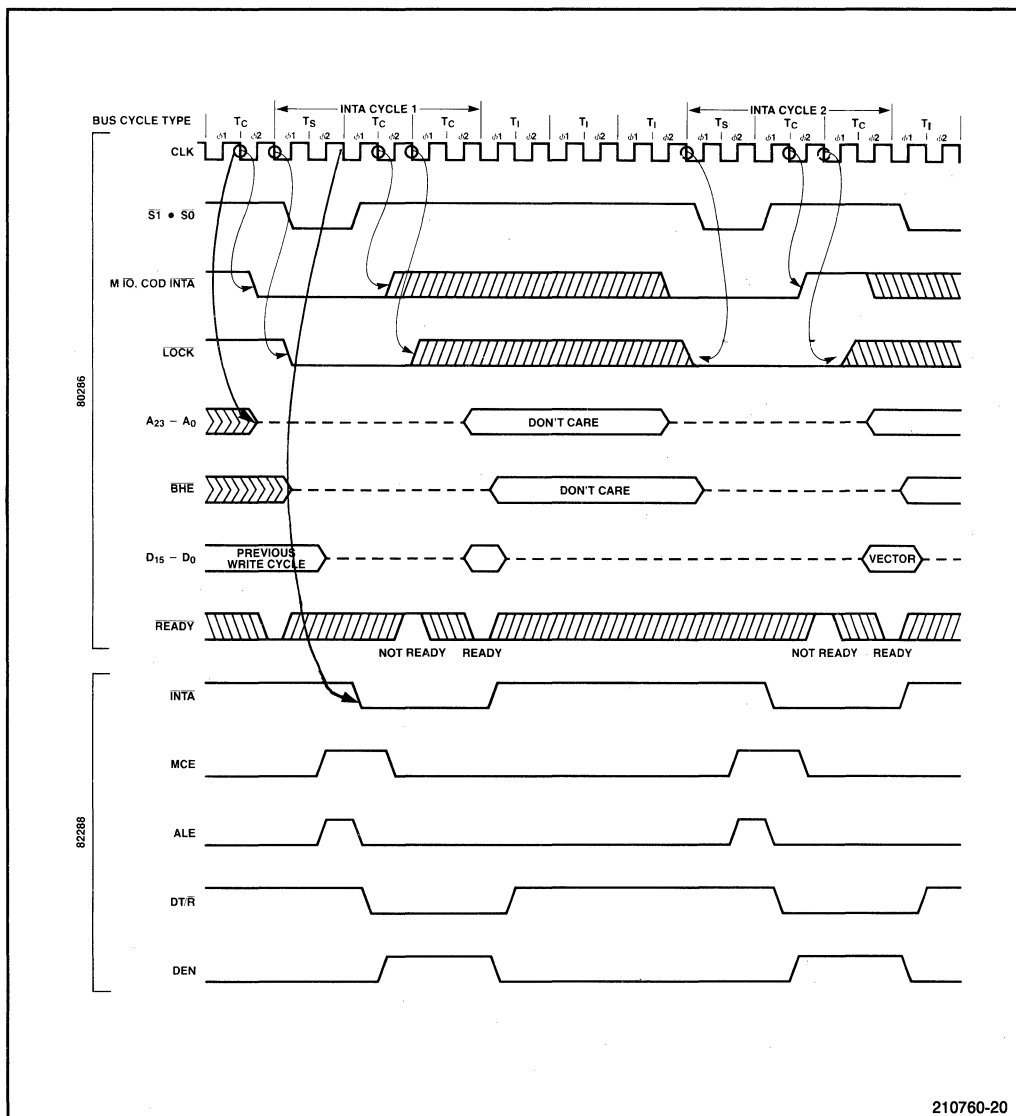
Figure 3-16. Interrupt-Acknowledge Sequence
