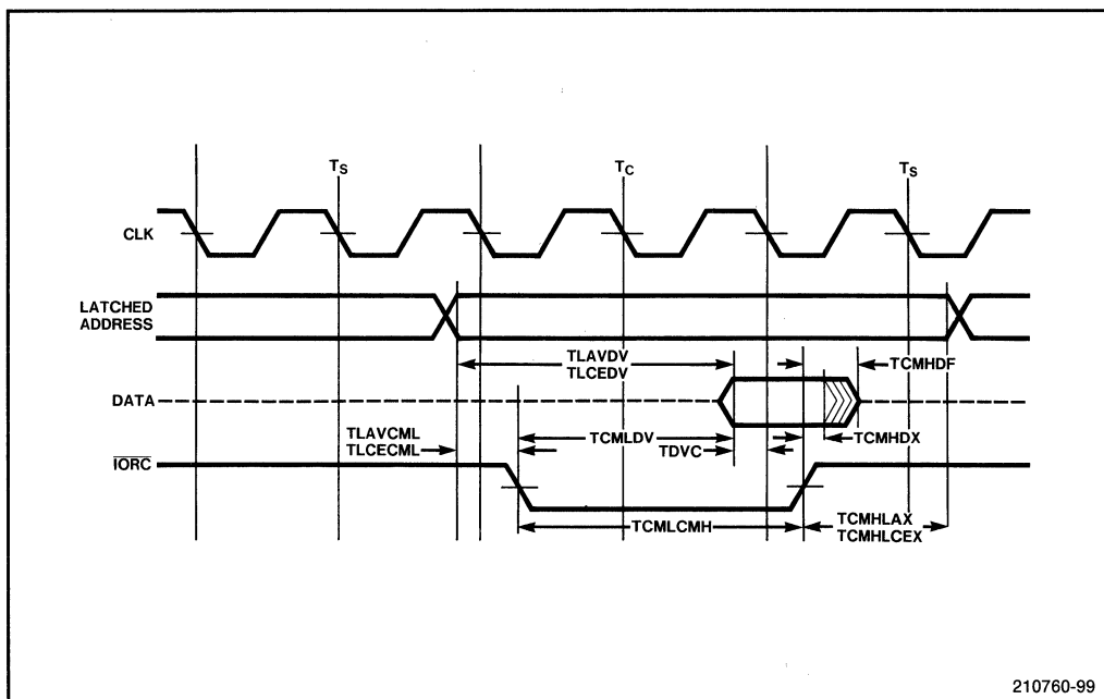
Figure 5-10. I/O Read Cycle Timing
