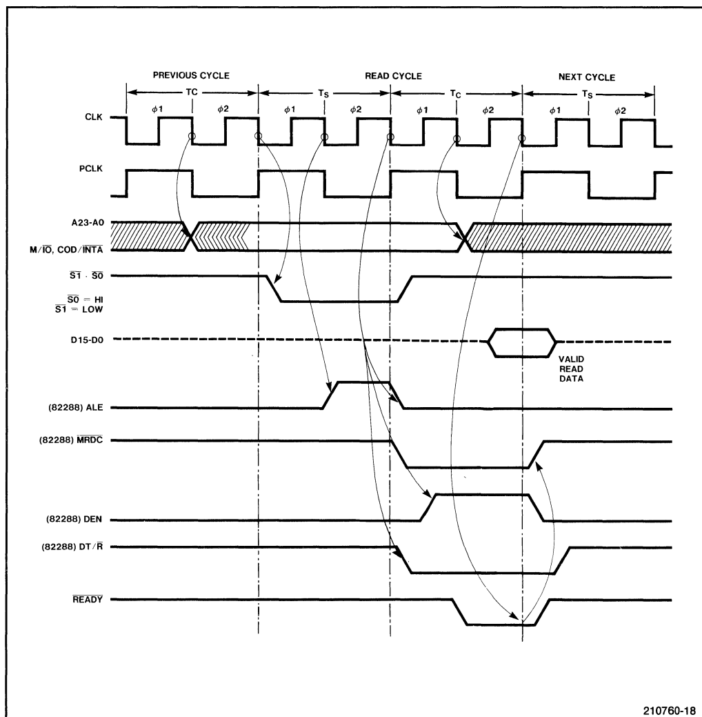
Figure 3-14. 80286 Read Cycle
