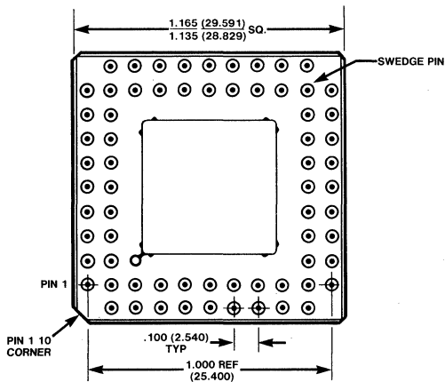
68-PIN CERAMIC PIN GRID ARRAY
