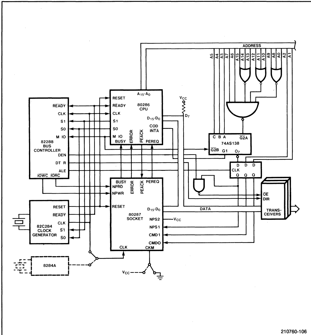
Figure 6-1. 80286/20 System Configuration
