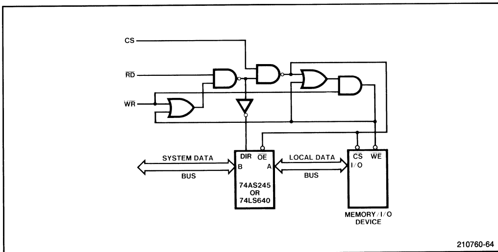
Figure 3-61. Buffering Devices without \overline{OE}/\overline{RD} and with Common or Separate Input/Output
