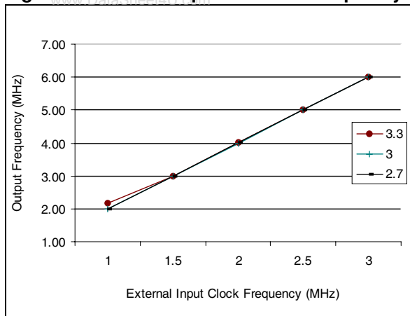
Figure 53. PLLx4 Output vs CLKIN frequency
