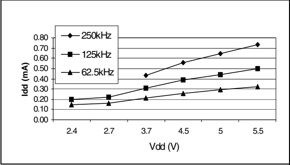
Figure 56. Typical I DD in SLOW vs. f CPU
