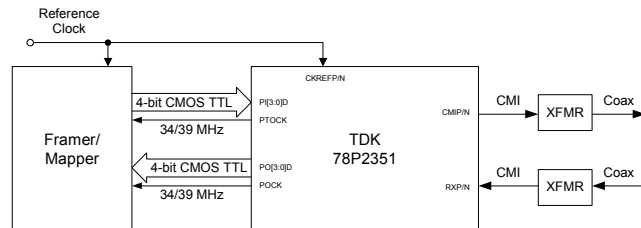
Figure 5: Master Parallel Mode
