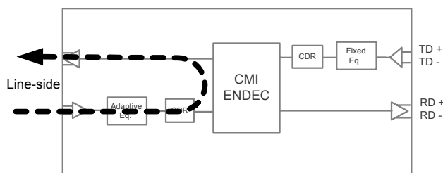
Figure 3: Remote (analog) Loopback
