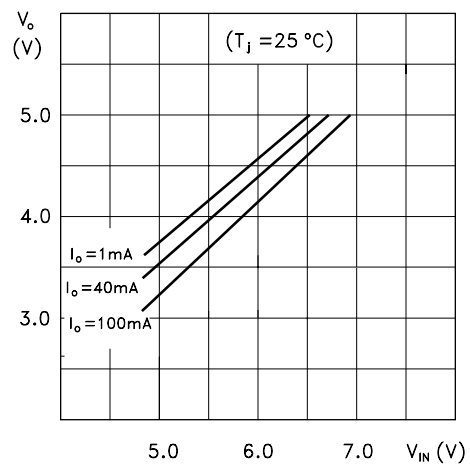
Figure 8 : Dropout Characteristics
