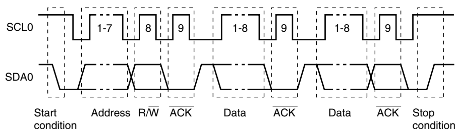
Figure 18-12. I 2 C Bus Serial Data Transfer Timing
