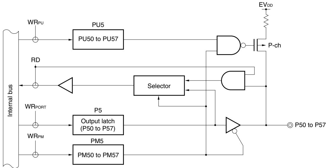
Figure 5-15. Block Diagram of P50 to P57
