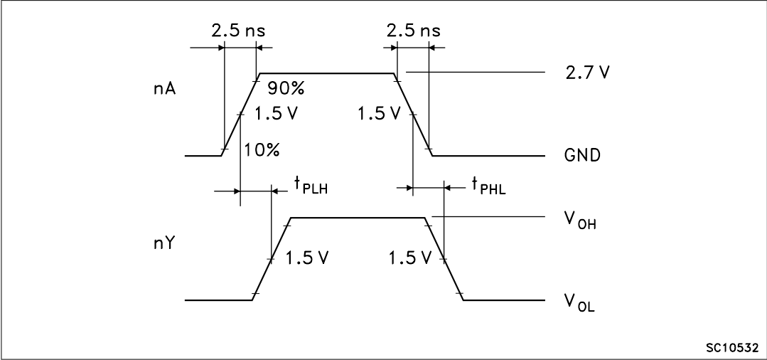
Figure 5. Propagation delay (f = 1 MHz; 50% duty cycle)
