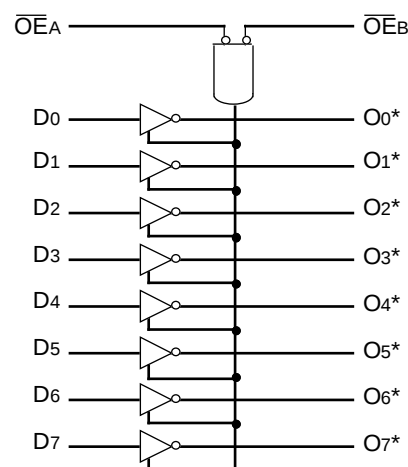
IDT54/74FCT540/541
