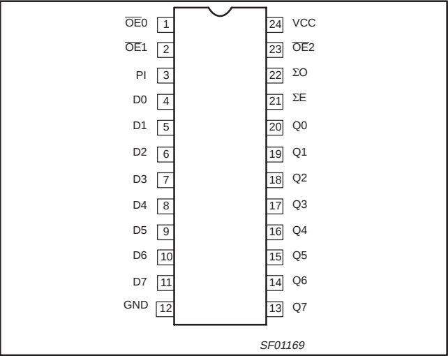
PIN CONFIGURATION – 74F656A
