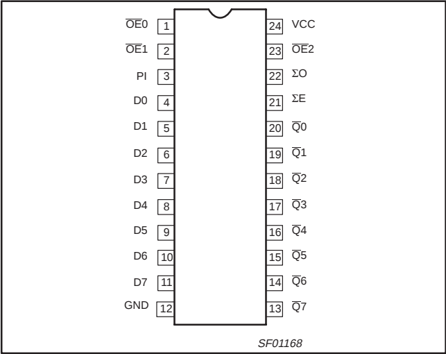
PIN CONFIGURATION – 74F655A
