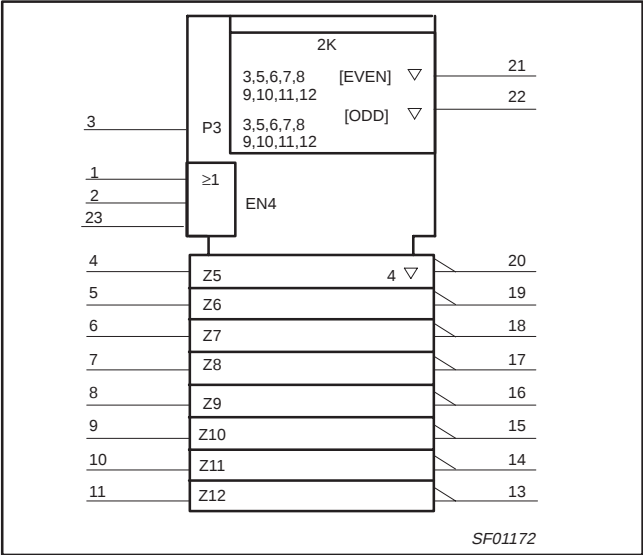
IEEE/IEC SYMBOL – 74F655A
