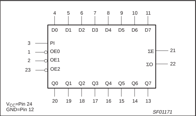
LOGIC SYMBOL – 74F656A
