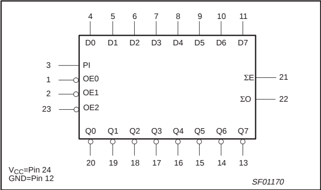
LOGIC SYMBOL – 74F655A
