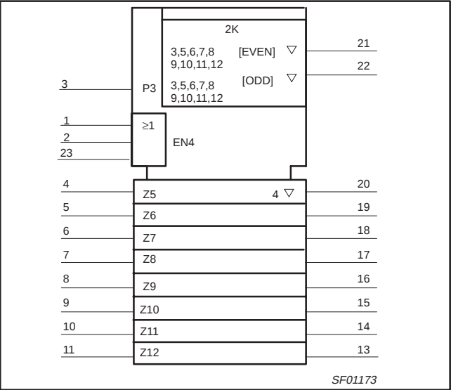
LOGIC SYMBOL (IEEE/IEC) – 74F656A
