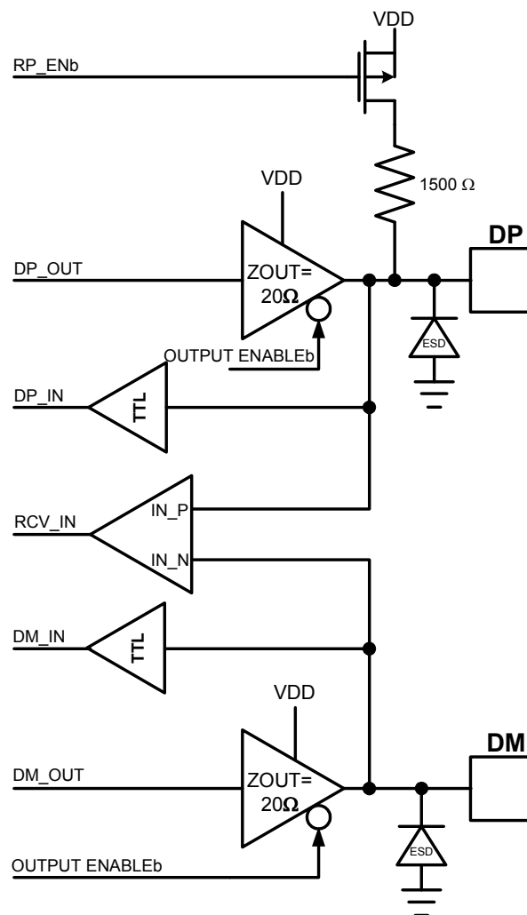
Figure 45: USB Circuit
