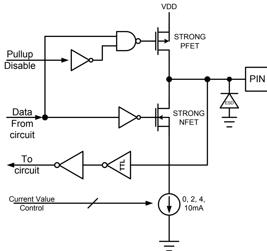
Figure 39: LED Circuit
