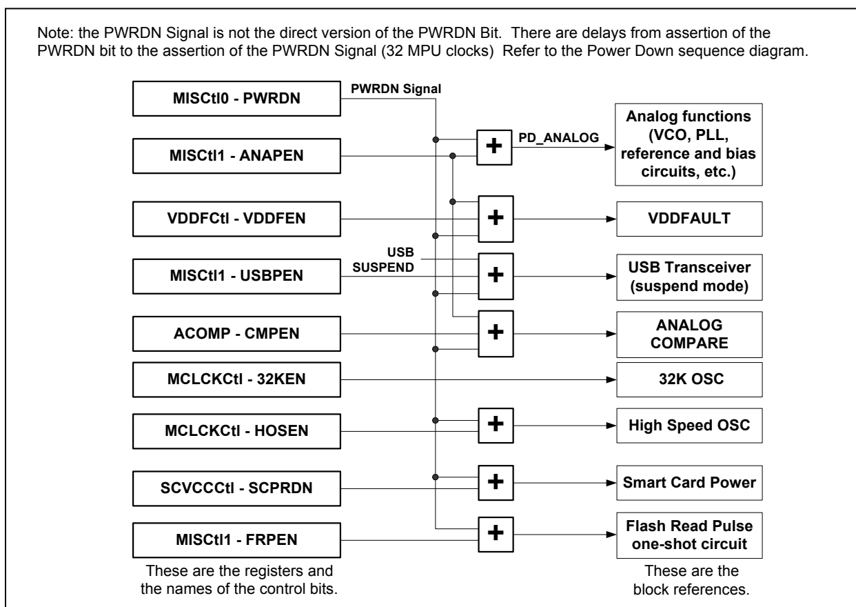
Figure 6: Power-Down Control
