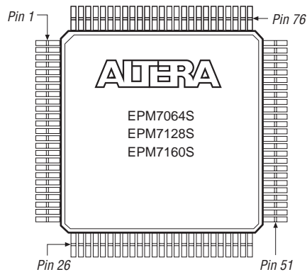
100-Pin TQFP
