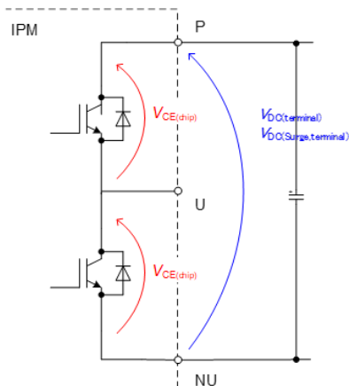
Fig.2-2 Rated Voltage
