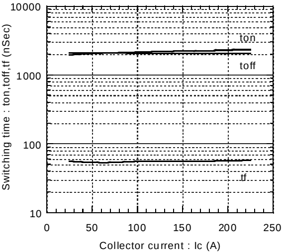
Switching time vs. Collector current Edc=300V,Vcc=15V,Tj=125°C
