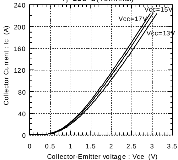
Collector current vs. Collector-Emitter voltage Tj=125°C(Terminal)
