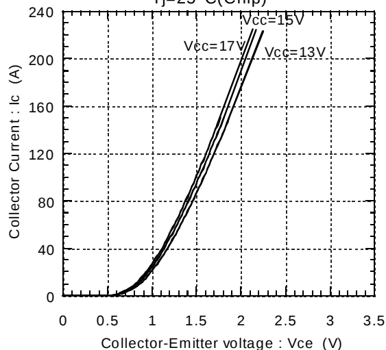
Collector current vs. Collector-Emitter voltage Tj=25°C(Chip)
