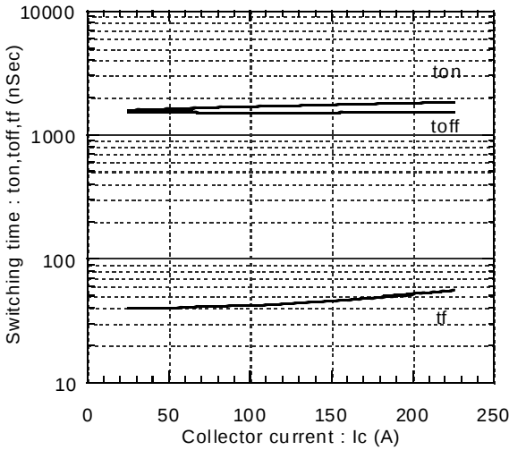
Switching time vs. Collector current Edc=300V,Vcc=15V,Tj=25°C
