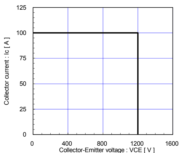
Reverse bias safe operating area (max.) +VGE=15V, -VGE ≤ 15V, RG ≥ 22Ω, Tj ≤ 125°C
