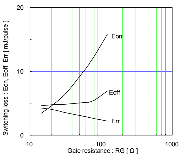
Switching loss vs. Gate resistance (typ.) Vcc=600V, Ic=50A, VGE=±15V, Tj=125°C
