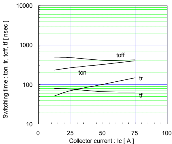
Switching time vs. Collector current (typ.) Vcc=600V, VGE=±15V, RG=22Ω, Tj=25°C
