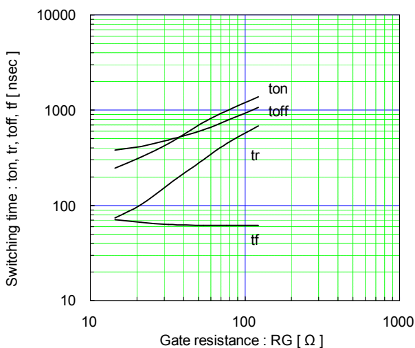
Switching time vs. Gate resistance (typ.) Vcc=600V, Ic=50A, VGE=±15V, Tj=25°C
