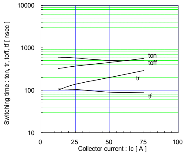
Switching time vs. Collector current (typ.) Vcc=600V, VGE=±15V, RG=22Ω, Tj=125°C
