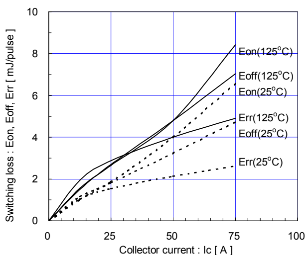
Switching loss vs. Collector current (typ.) Vcc=600V, VGE=±15V, RG=22Ω
