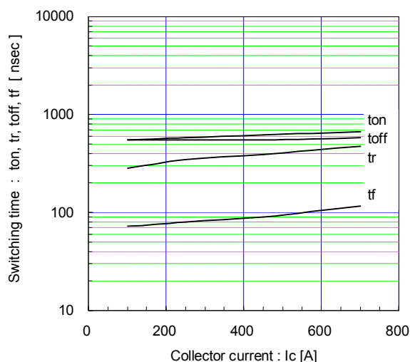
Switching time vs. Collector current (typ.) V_{CC}=900V , V_{GE}=\pm 15V , R_g=1.1\Omega , T_j=25^\circ C
