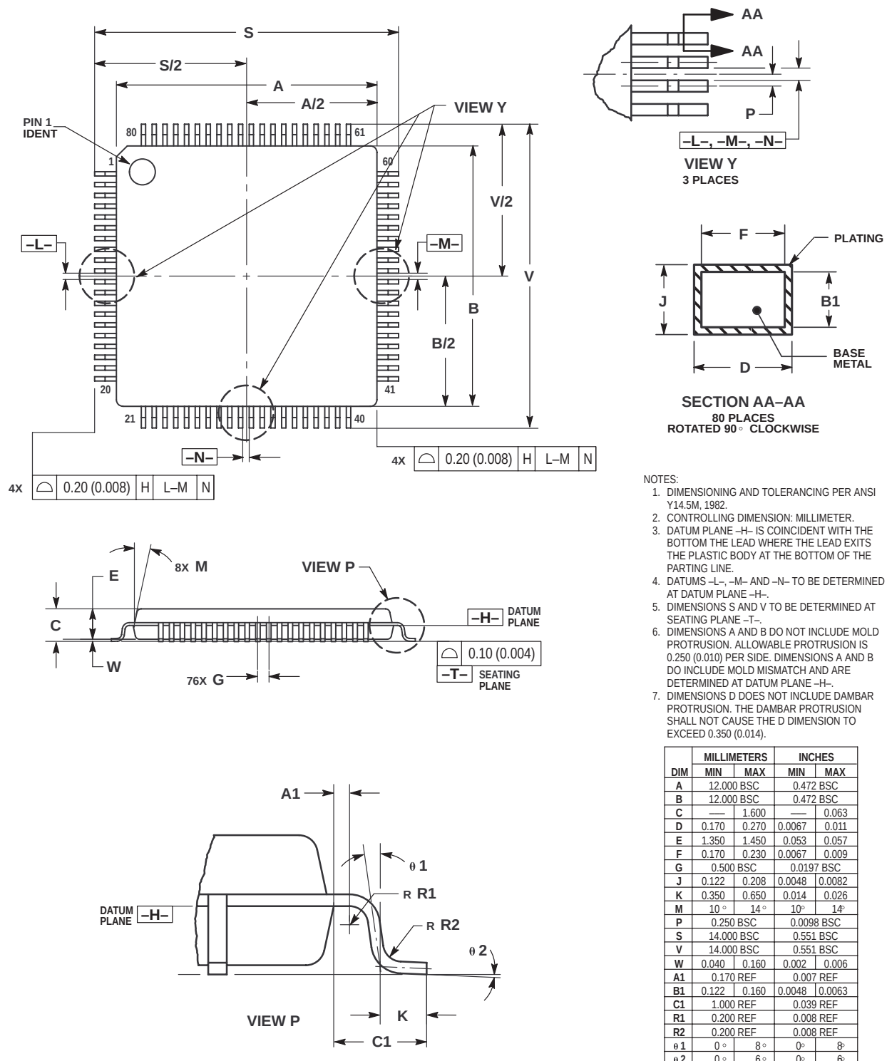
Figure 15-1. 80-Pin TQFP Mechanical Dimensions
