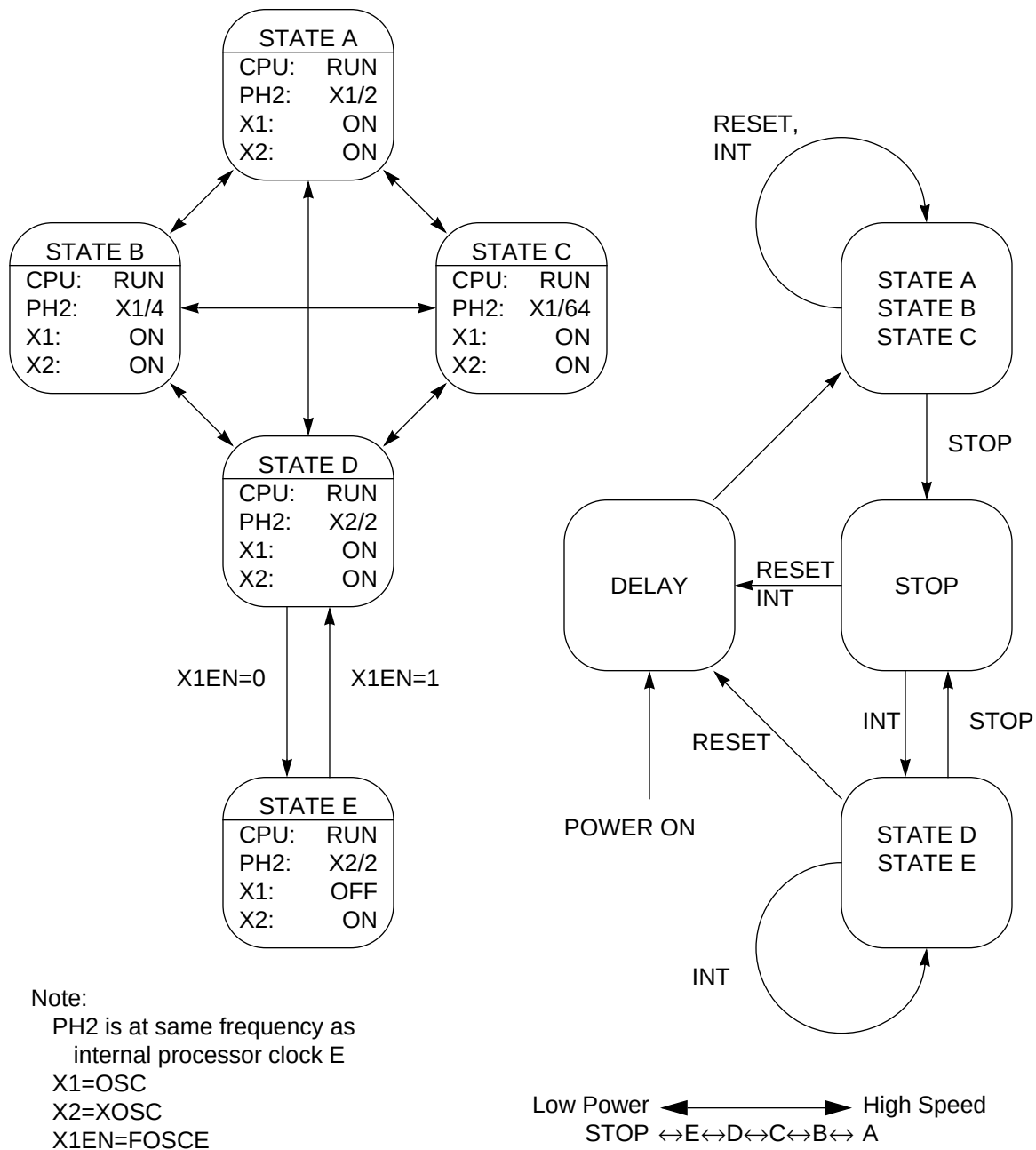
Figure 6-1. Clock State and STOP Recovery/POR Delay Diagrams
