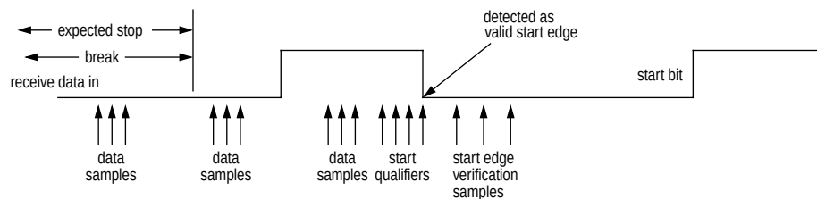
Figure 11-6. SCI Start following a Break
