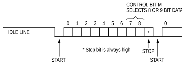
Figure 11-2. Data Format
