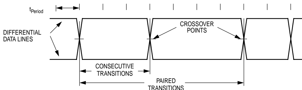
Figure 10-14. Data Jitter
