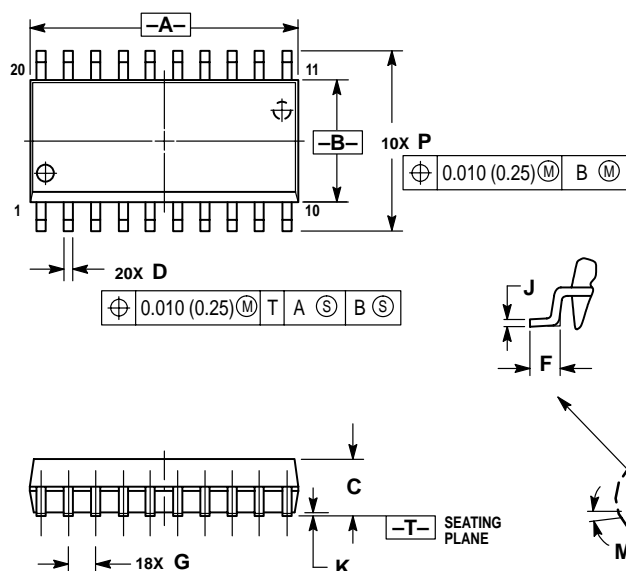
Figure 14-3. 20-Pin SOIC Mechanical Dimensions
