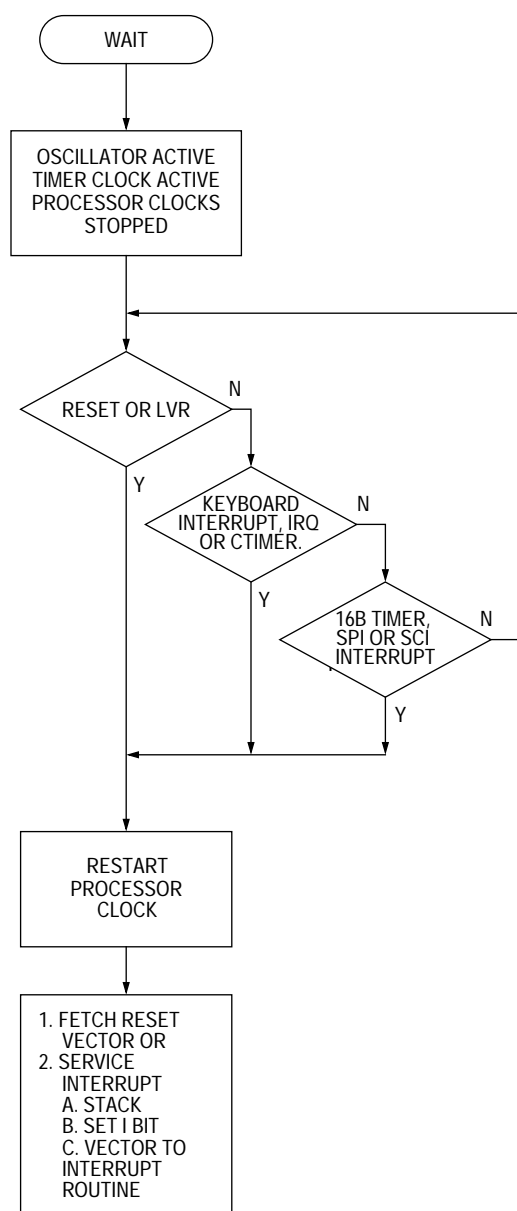
Figure 6-1. WAIT Flowchart
