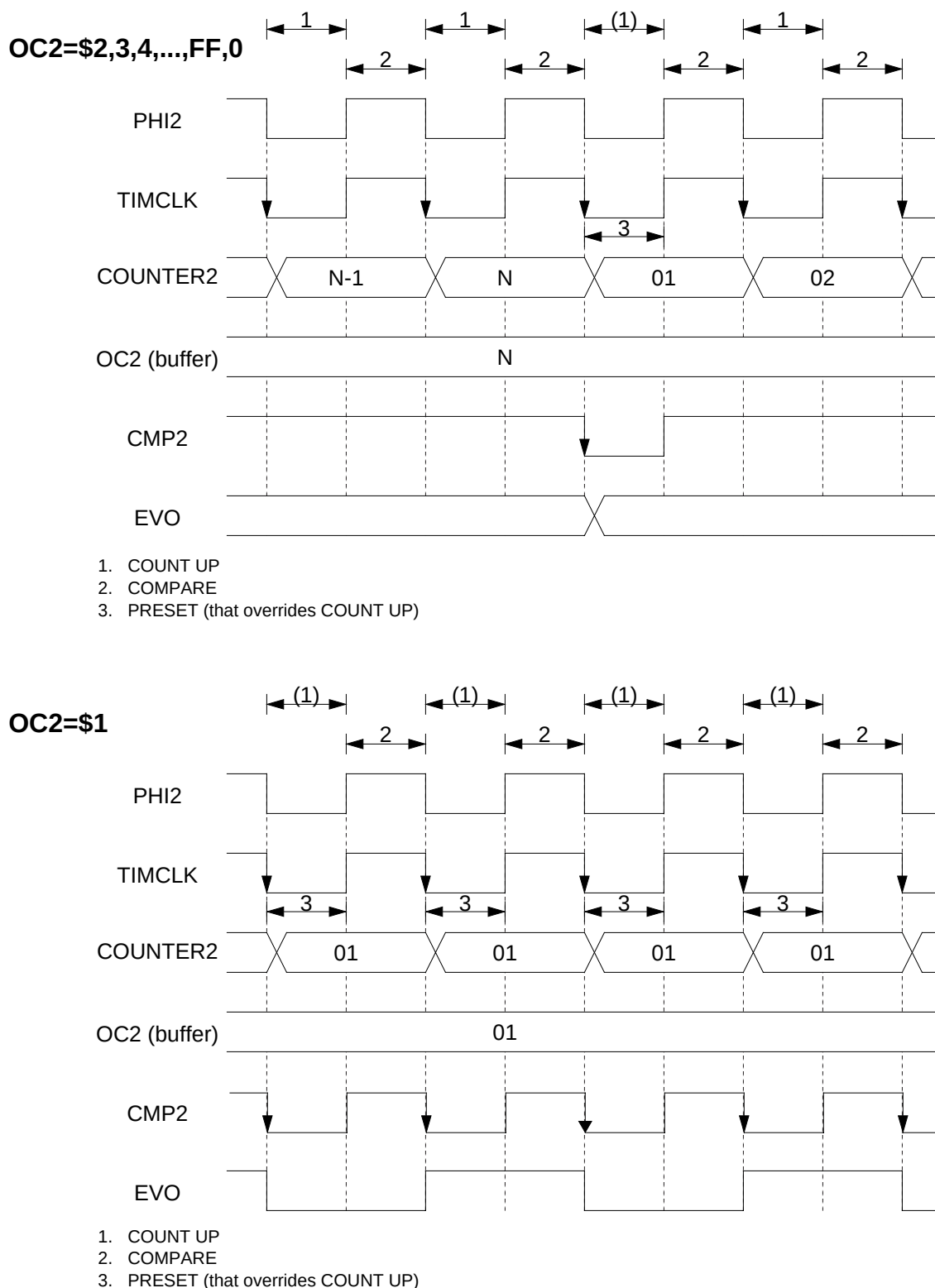
Figure 8-5: Timer 2 Timing for f(\text{PHI2}) = f(\text{TIMCLK})
