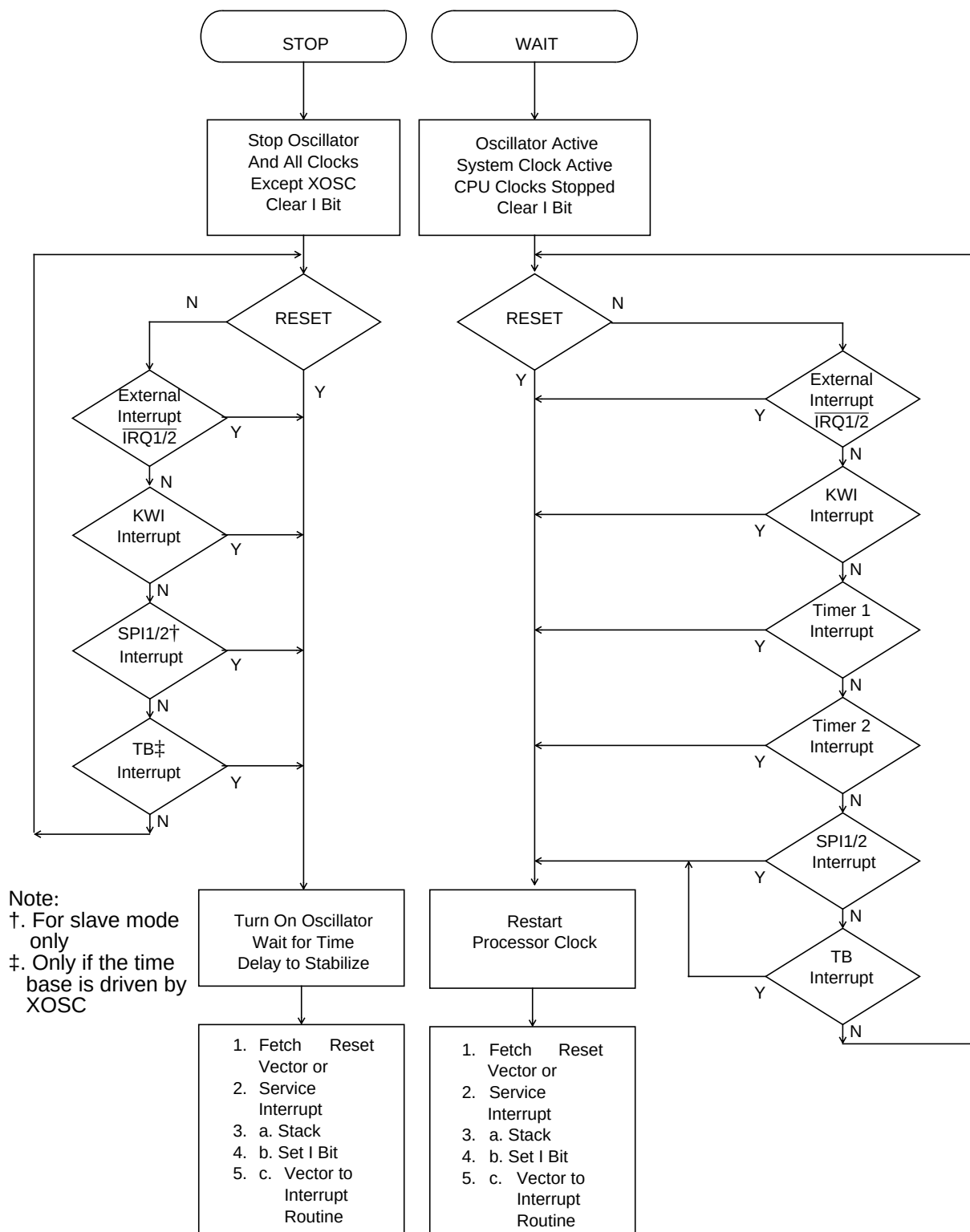
Figure 4-3: STOP/WAIT Flowcharts
