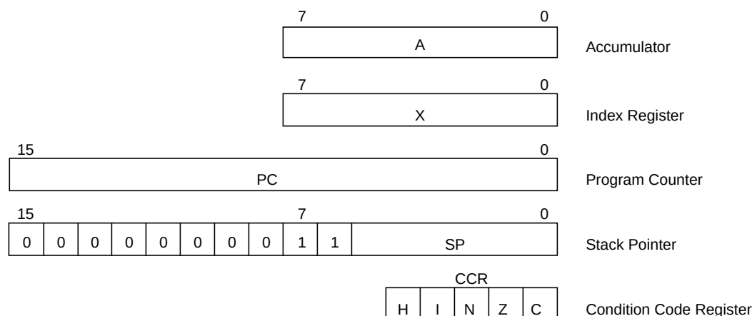
Figure 4-1: Programming Model
