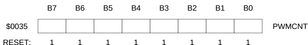
Figure 9-5: PWM Counter
