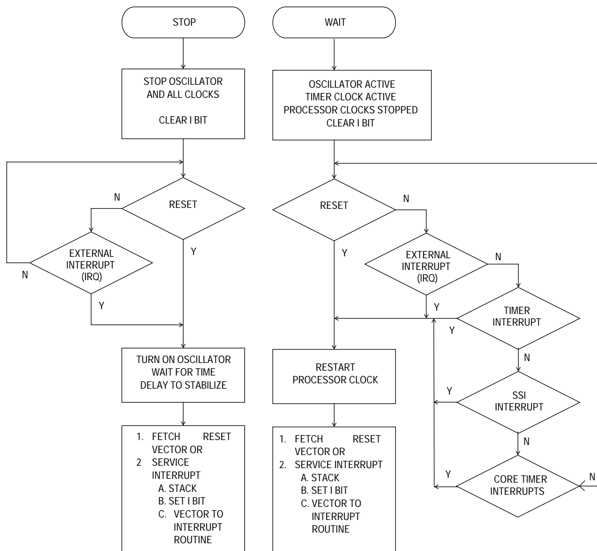
Figure 6-3. STOP/WAIT Flowchart
