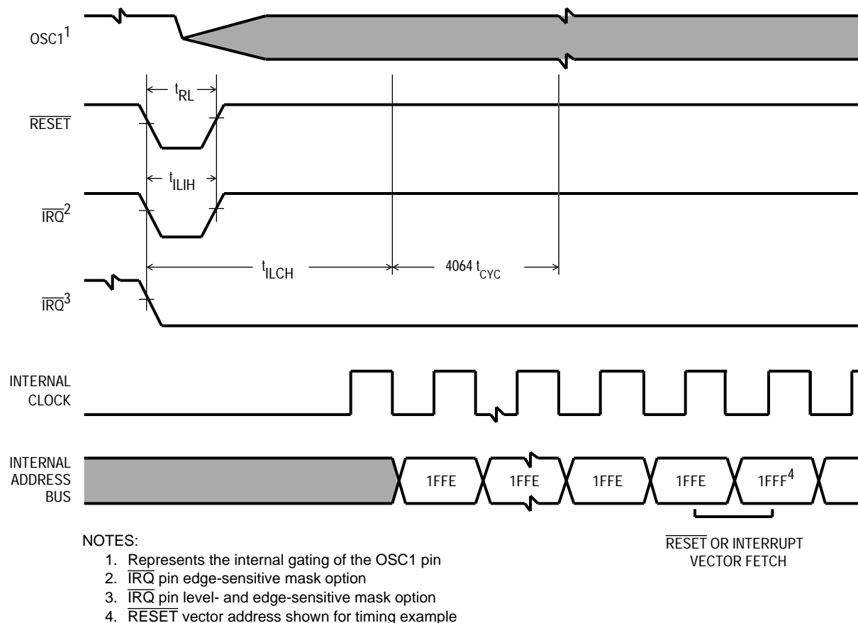
Figure 16-1. Stop Recovery Timing Diagram
