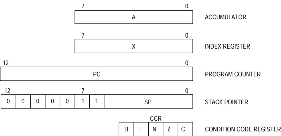
Figure 3-1. Programming Model
