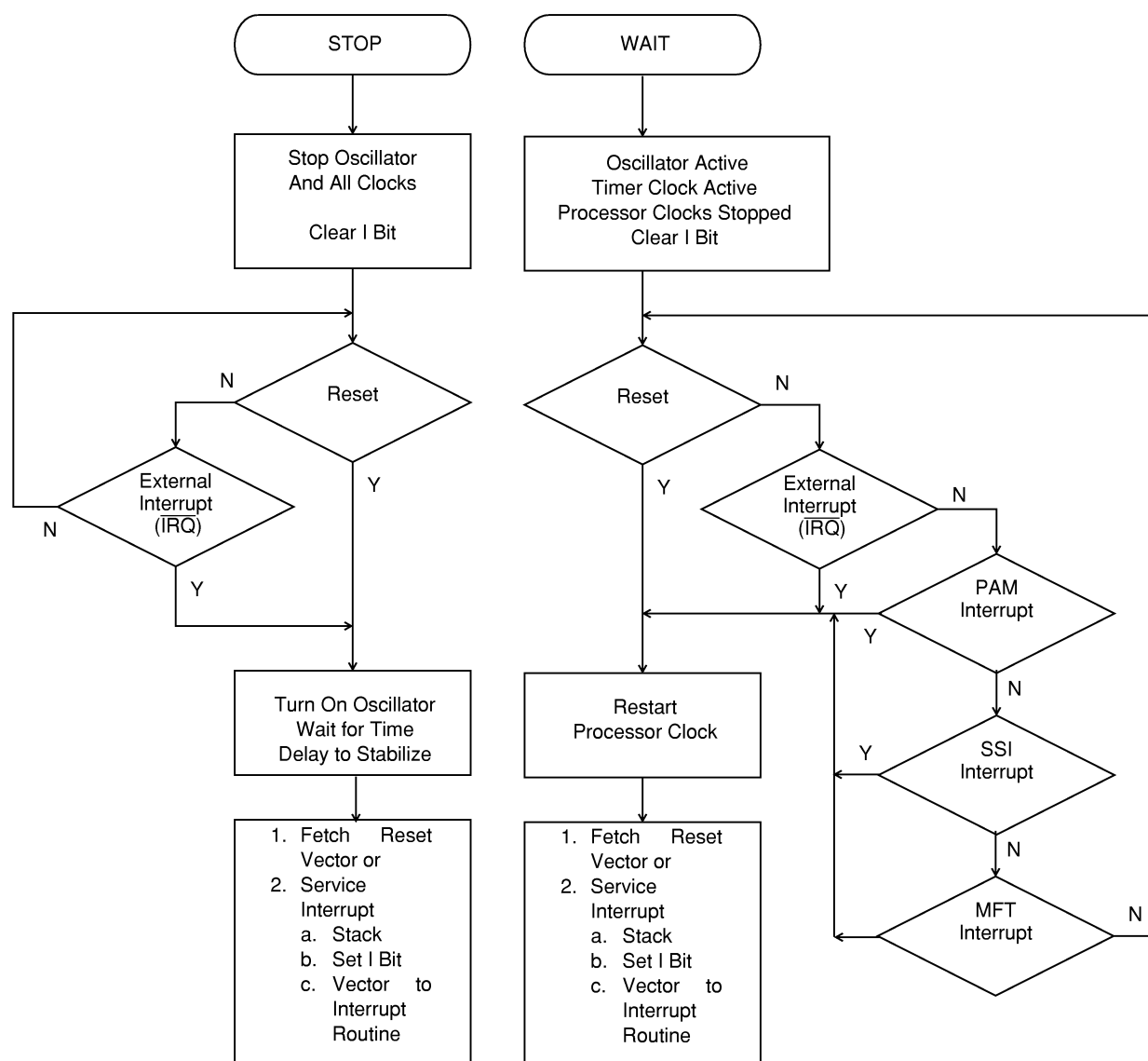
Figure 6-2. STOP/WAIT Flowchart
