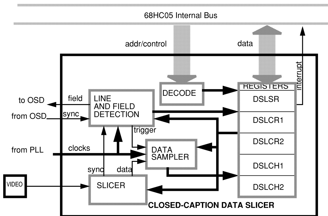
Figure 12-1. Data Slicer Block Diagram
