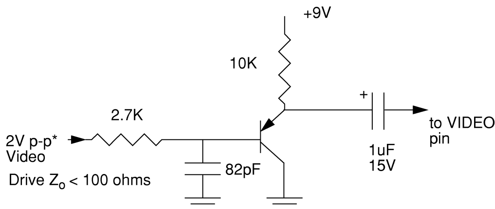
Figure 12-3. Video Input Circuit
