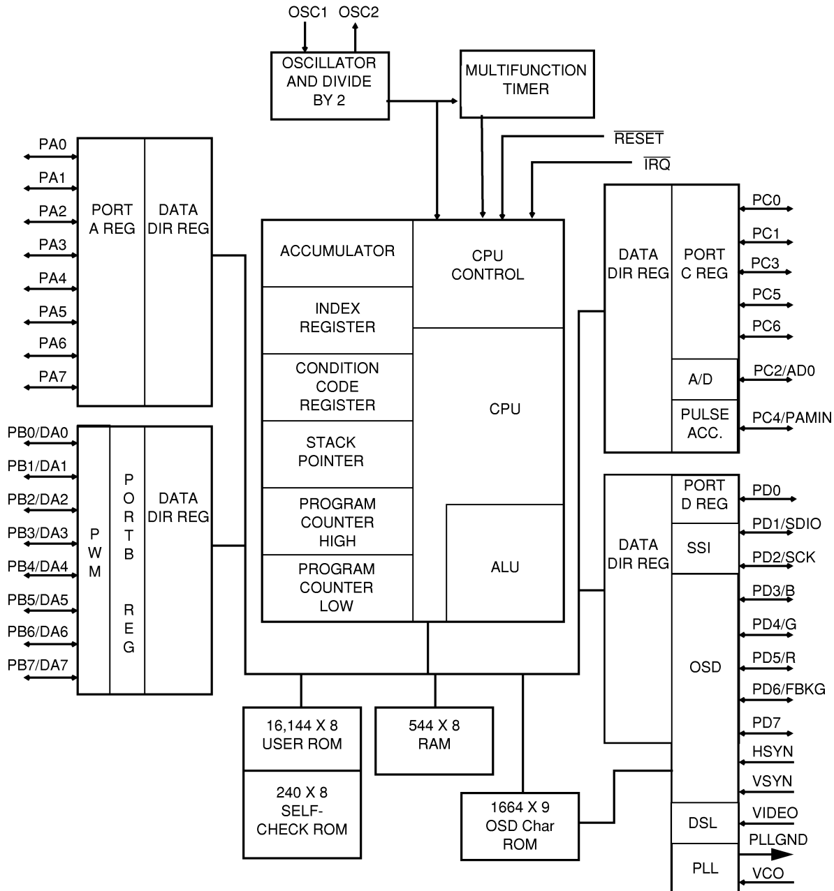
Figure 1-1. Block Diagram
