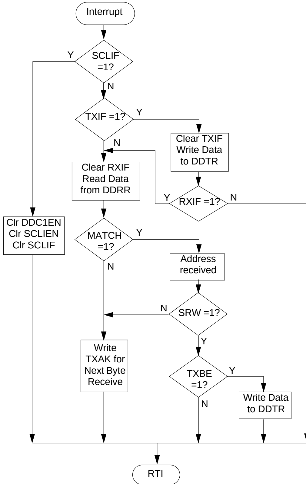
Figure 9-1: Software Flowchart of Slave Mode Interrupt Routine
