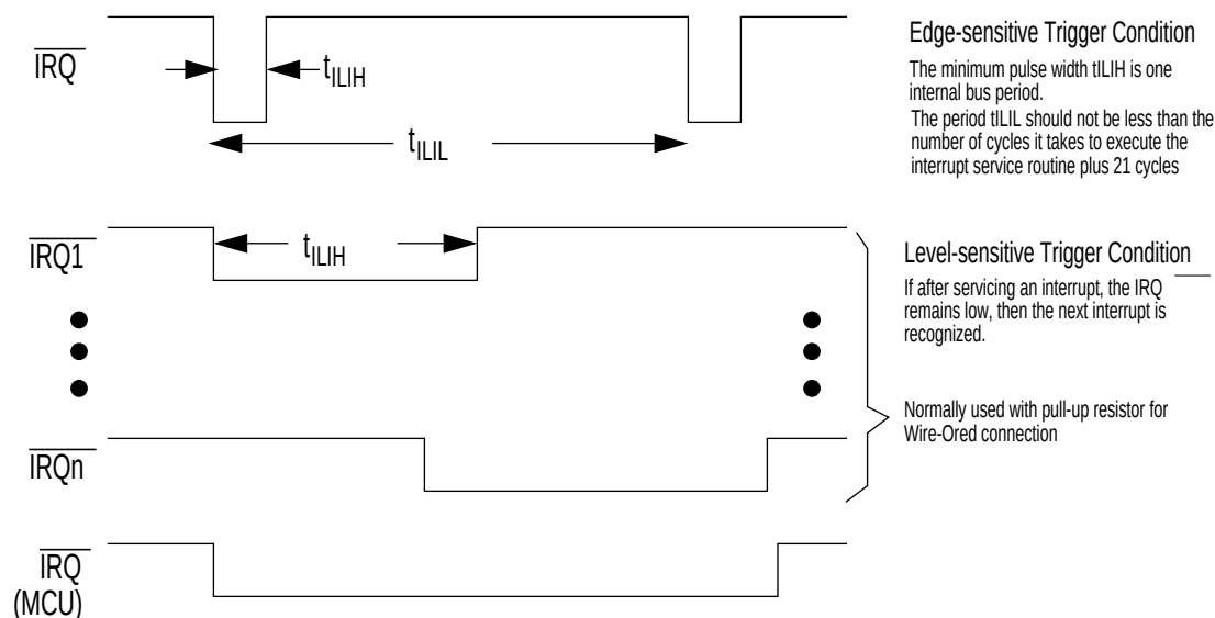
Figure 4-2: External Interrupt
