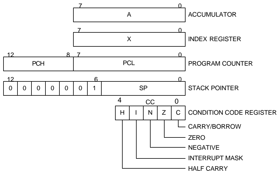
Figure 6. Programming Model
