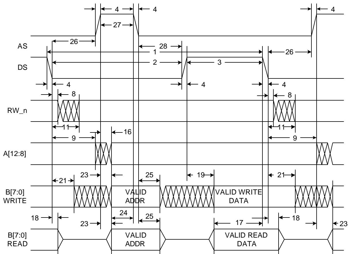
Figure 19. Bus Timing
