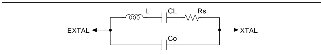
Figure 5.5 Crystal Oscillator Equivalent Circuit
