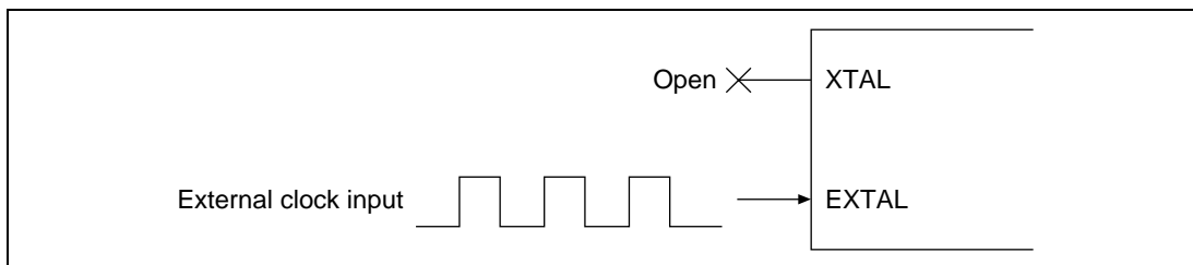
Figure 5.6 External Clock Input Method (Example)
