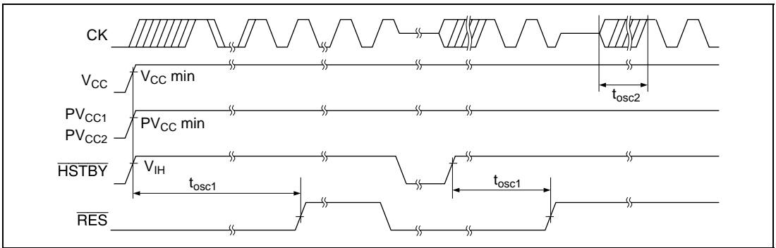
Figure 27.4 Oscillation Settling Time
