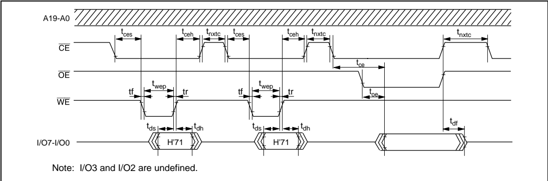
Figure 22.38 Timing in Status Read Mode
