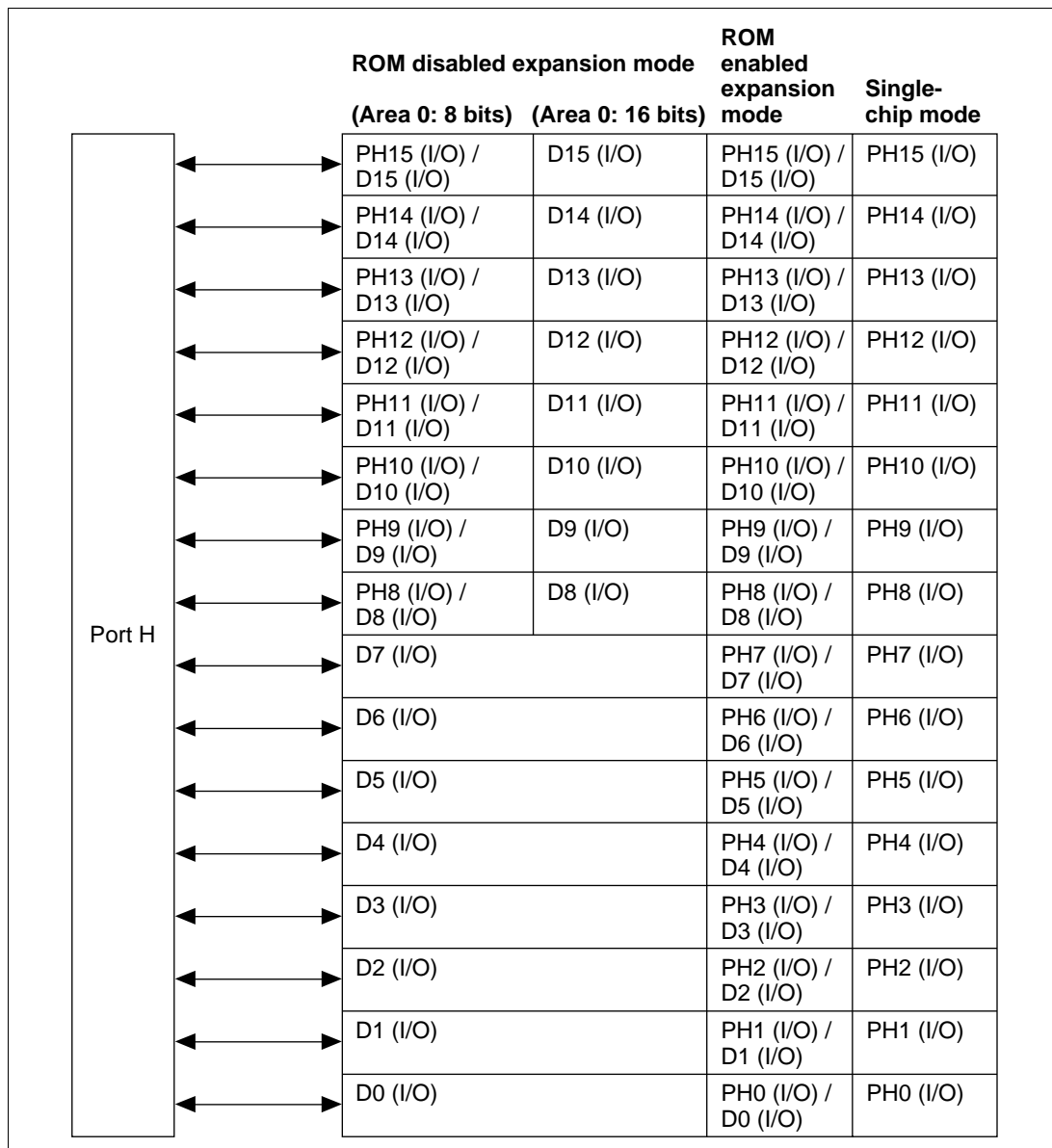
Figure 21.8 Port H
