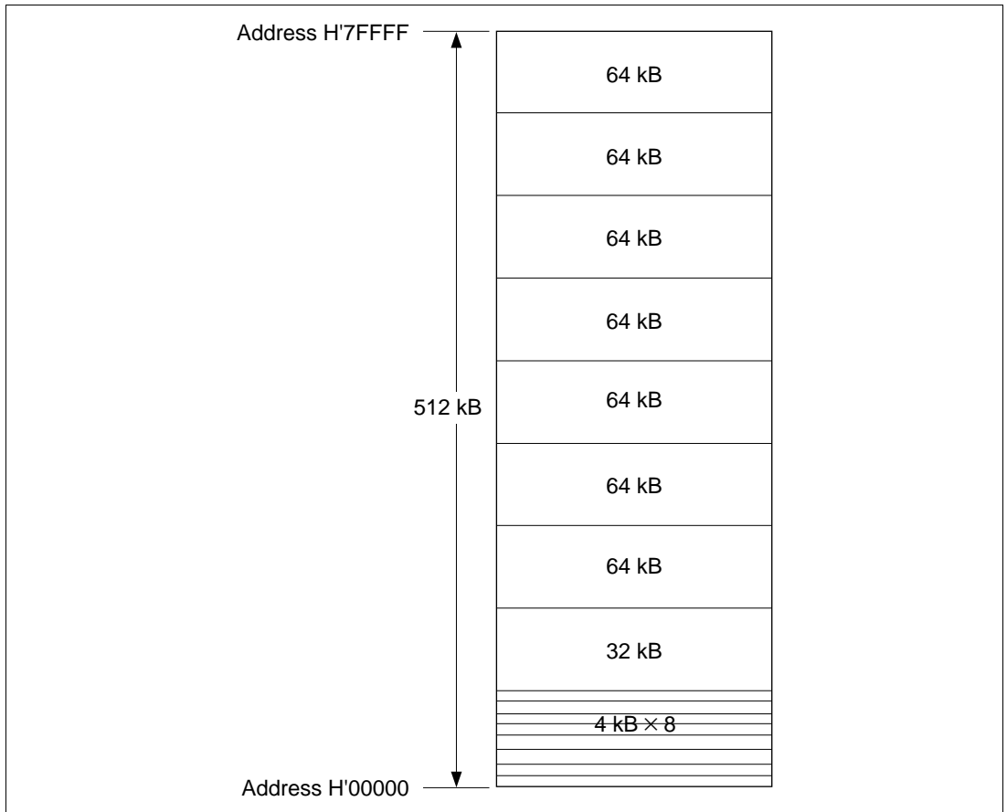
Figure 22.7 Block Configuration
