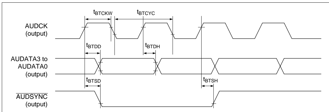
Figure 25.25 Branch Trace Timing
