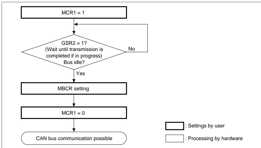
Figure 15.12 HCAN Halt Mode Flowchart
