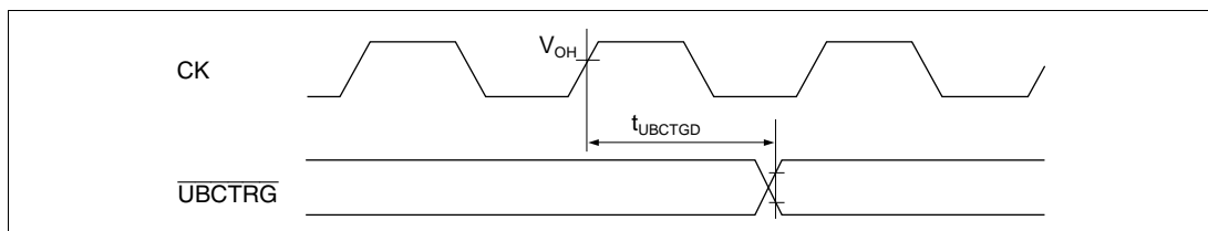
Figure 24.23 UBC Trigger Timing
