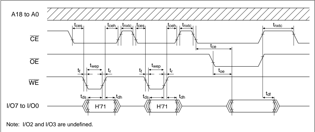
Figure 21.27 Status Read Mode Timing Waveforms
