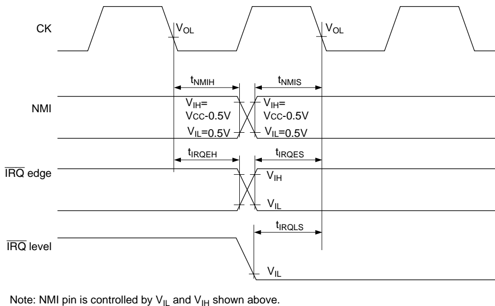
Figure 24.6 Interrupt Signal Input Timing
