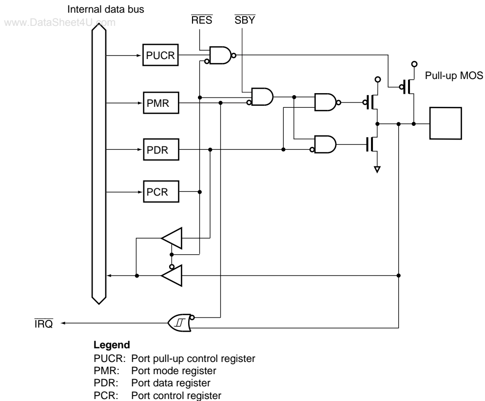
Figure B.2 Port 1 Block Diagram (P14)
