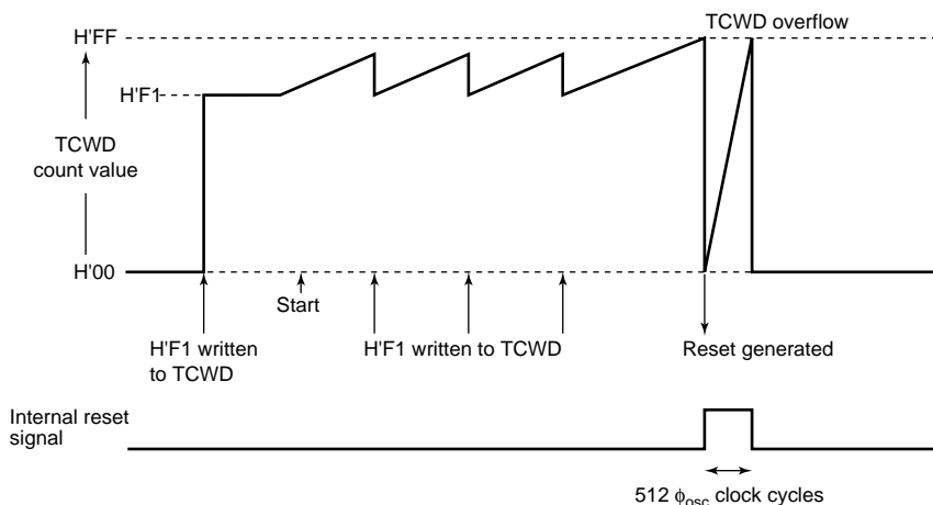
Figure 12.2 Watchdog Timer Operation Example
