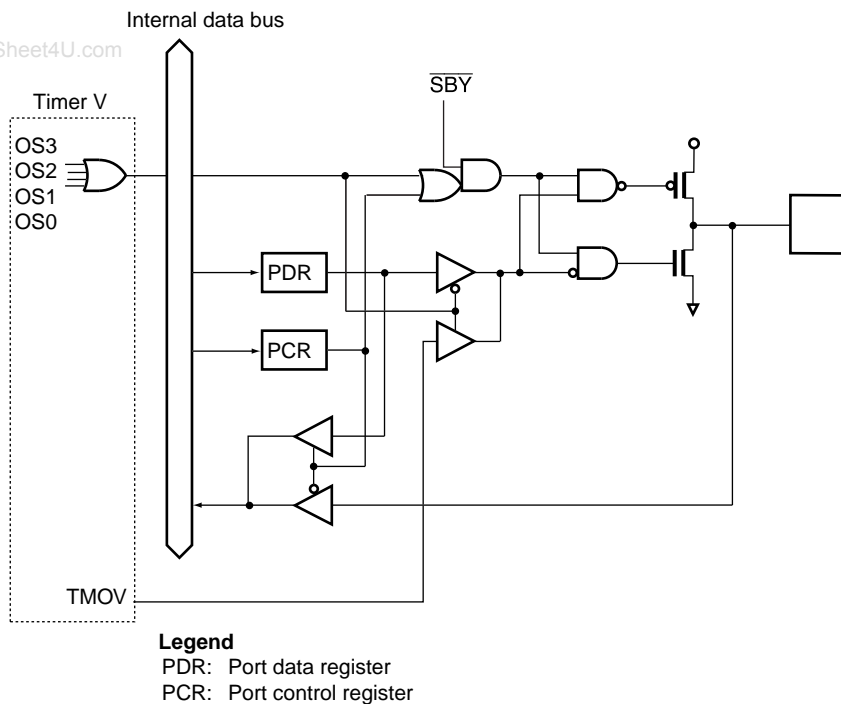
Figure B.11 Port 7 Block Diagram (P76)
