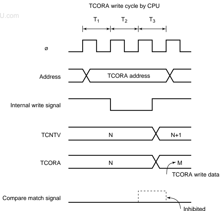
Figure 10.12 Contention between TCORA Write and Compare Match
