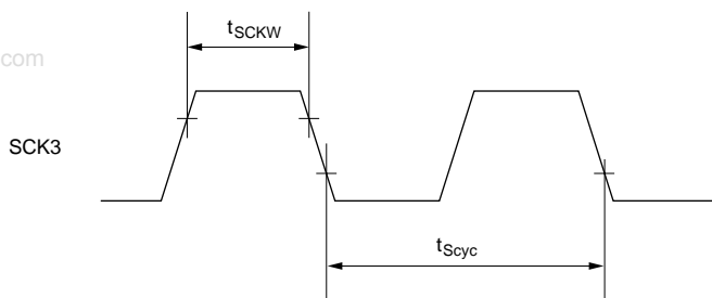
Figure 17.4 SCK3 Input Clock Timing
