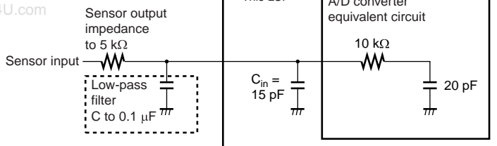
Figure 14.6 Analog Input Circuit Example
