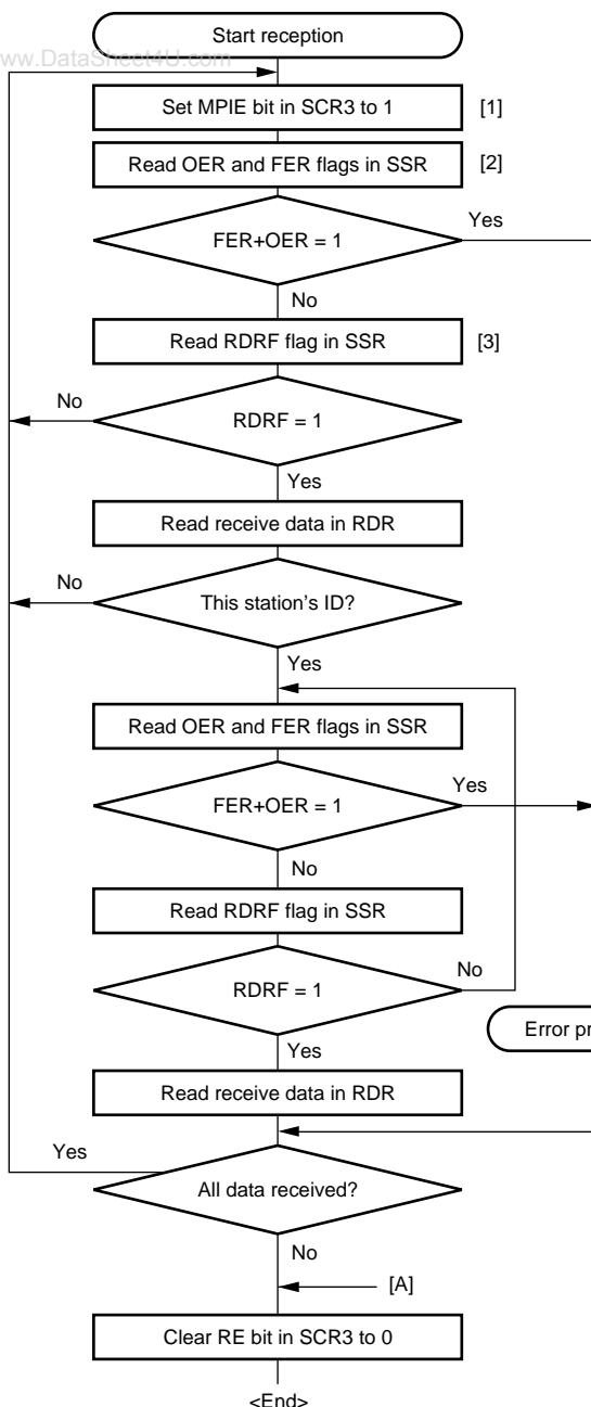
Figure 13.17 Sample Multiprocessor Serial Reception Flowchart (1)
