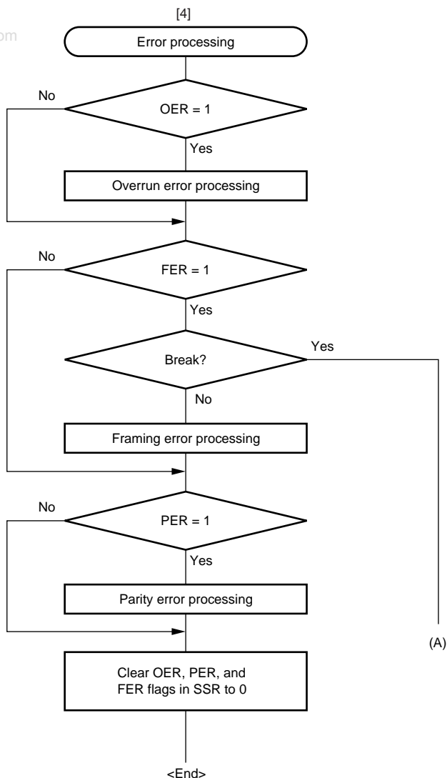
Figure 13.8 Sample Serial Reception Data Flowchart (2)
