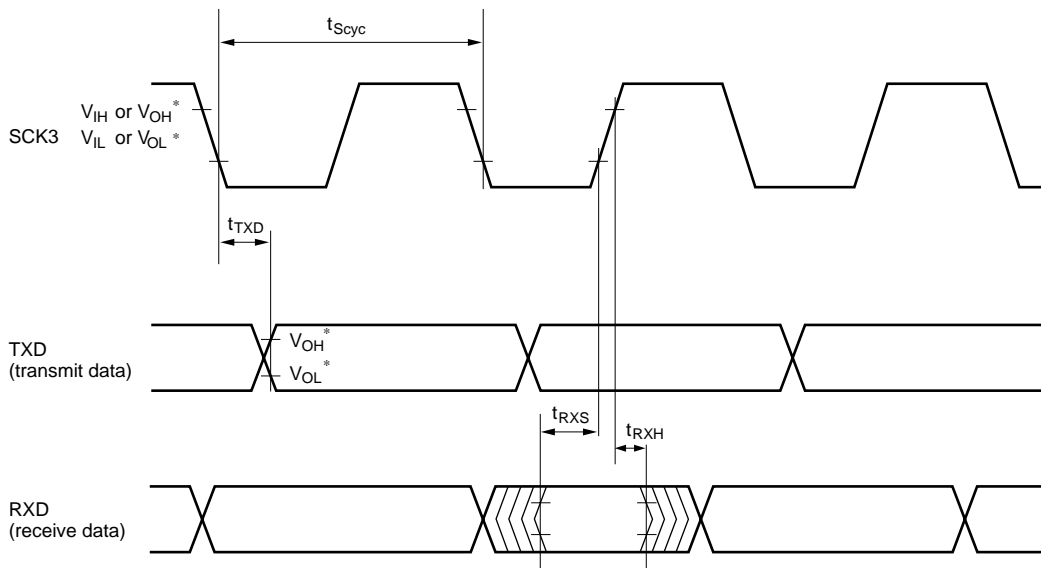
Figure 17.4 SCK3 Input Clock Timing
