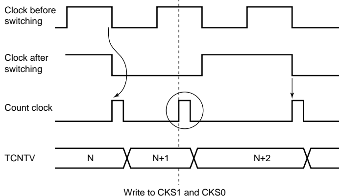
Figure 10.13 Internal Clock Switching and TCNTV Operation
