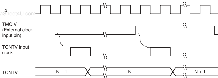
Figure 11.3 Increment Timing with External Clock
