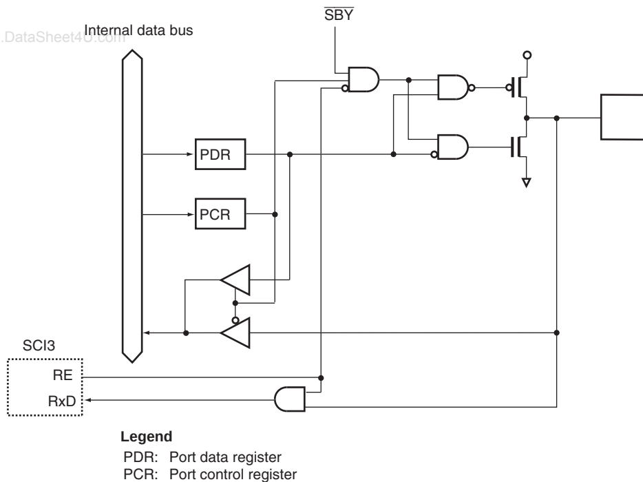
Figure B.6 Port 2 Block Diagram (P21)
