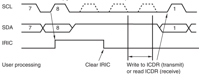
Figure 15.11 IRIC Setting Timing and SCL Control
