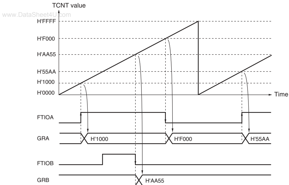
Figure 12.7 Input Capture Operating Example
