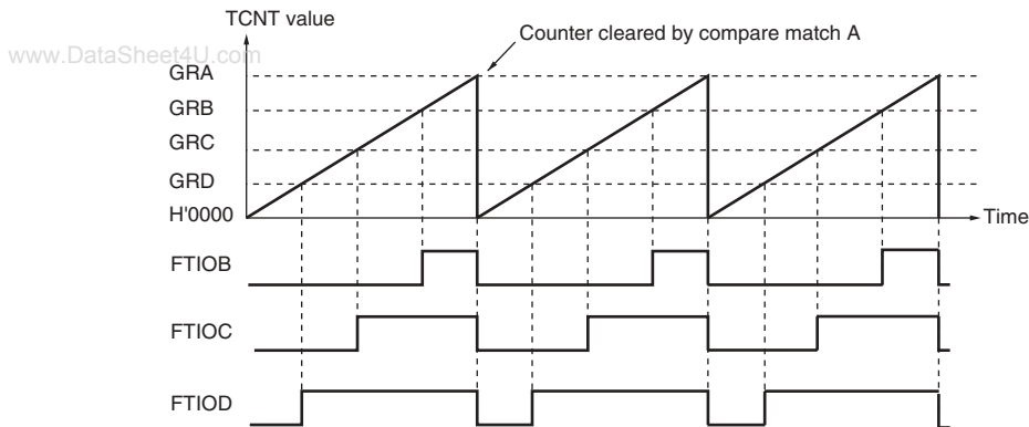
Figure 12.10 PWM Mode Example (2)
