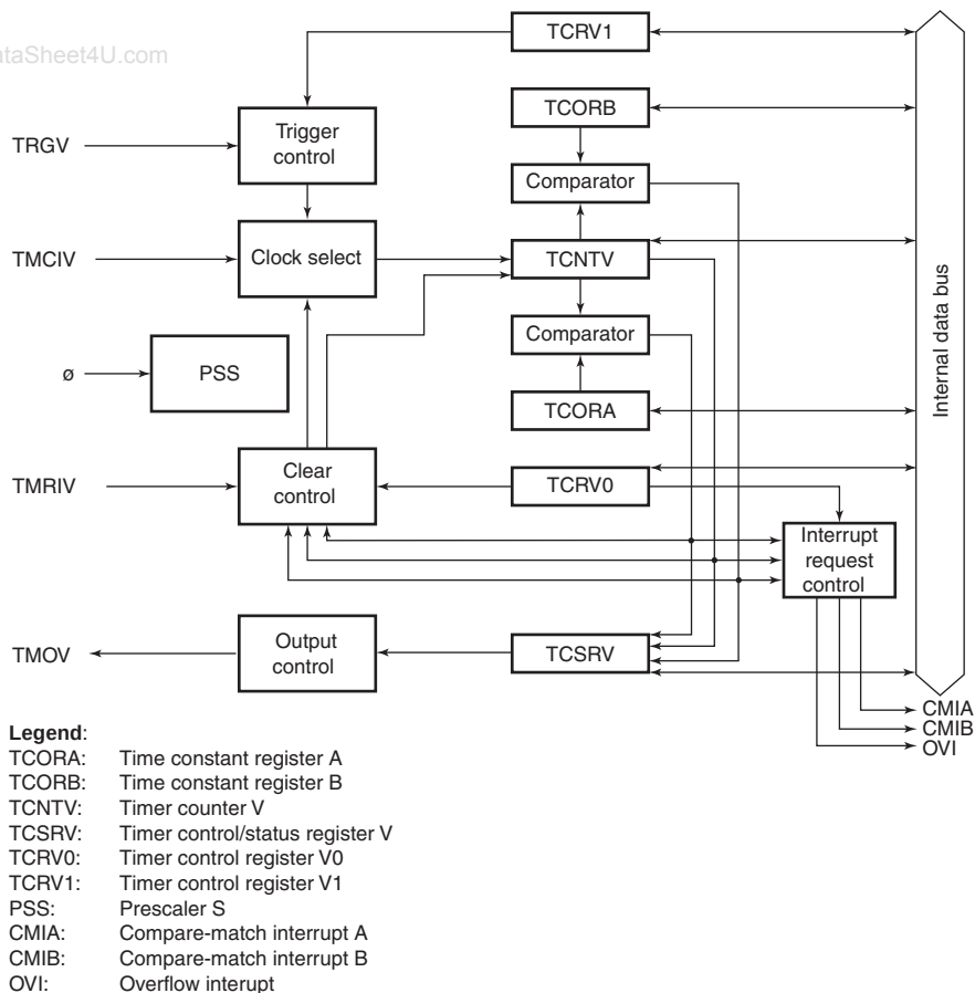
Figure 11.1 Block Diagram of Timer V
