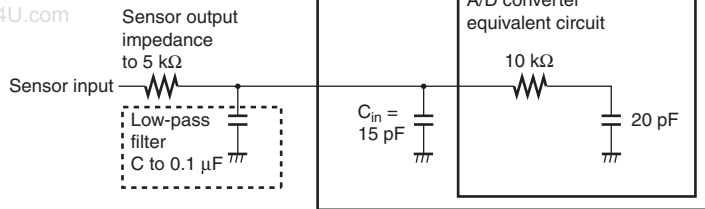
Figure 16.6 Analog Input Circuit Example
