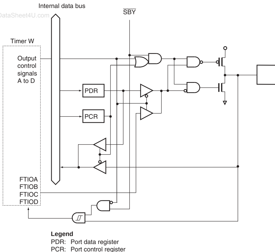
Figure B.15 Port 8 Block Diagram (P84 to P81)
