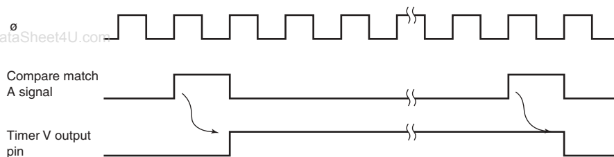
Figure 11.6 TMOV Output Timing
