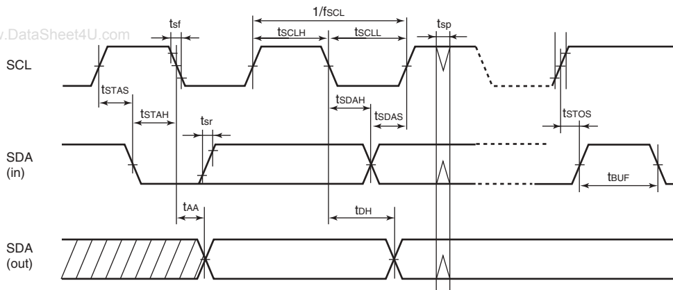
Figure 20.7 EEPROM Bus Timing
