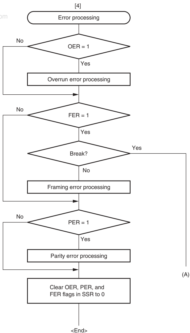
Figure 14.8 Sample Serial Reception Data Flowchart (2)
