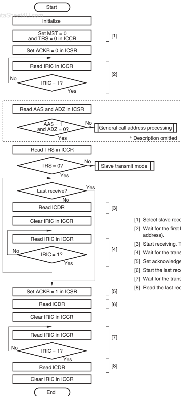
Figure 15.15 Sample Flowchart for Slave Receive Mode
