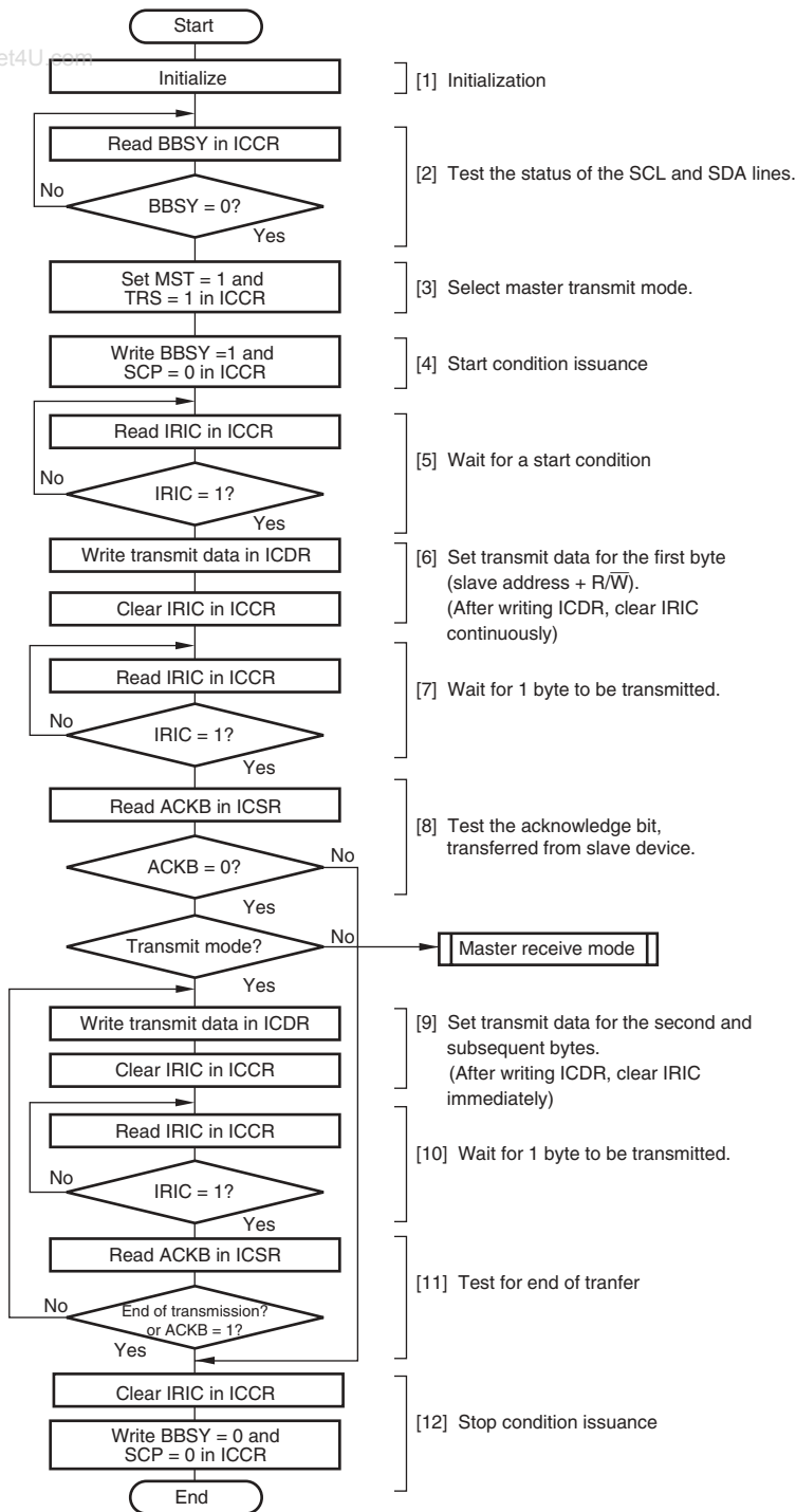
Figure 15.13 Sample Flowchart for Master Transmittion Mode
