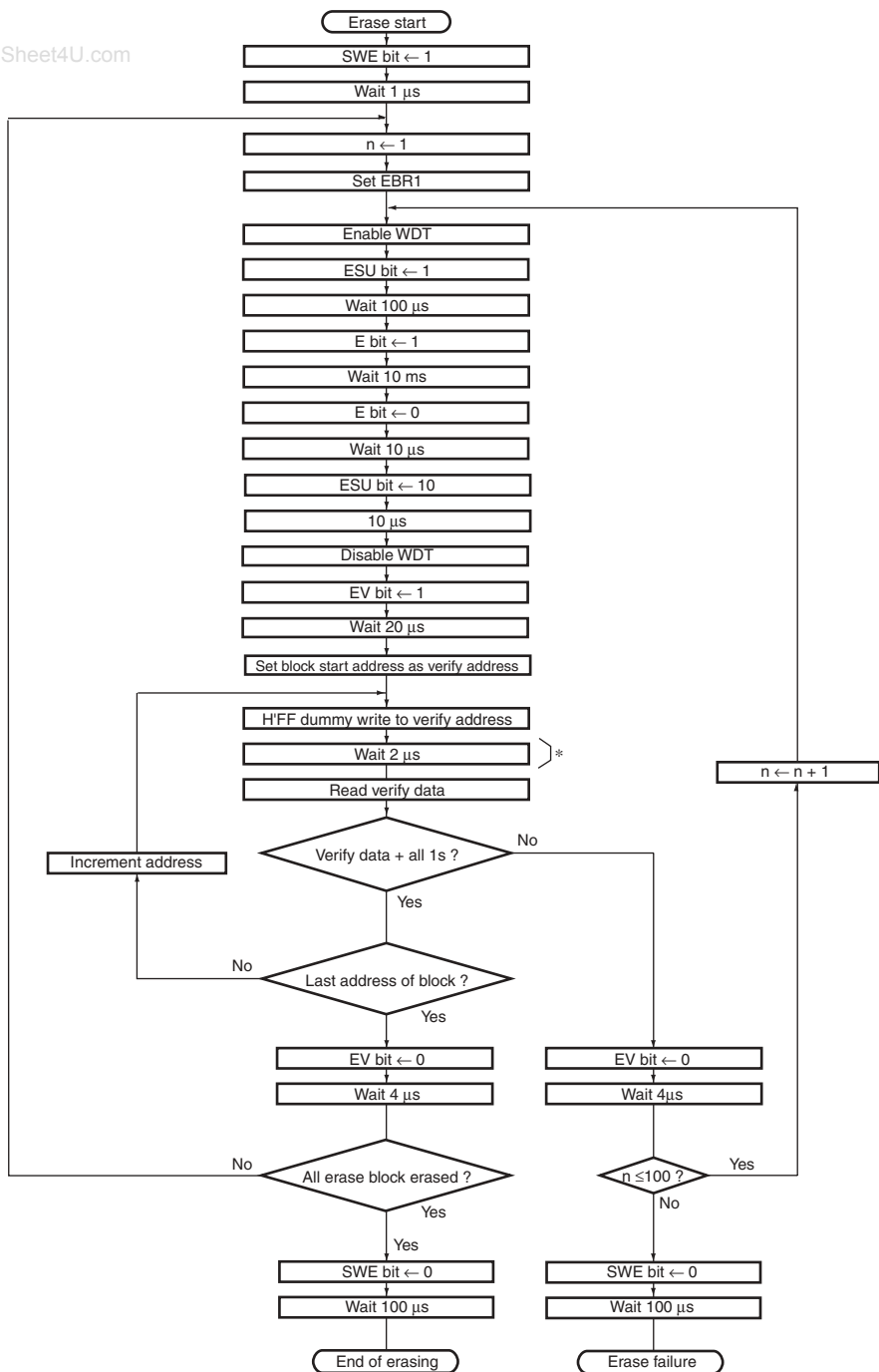
Figure 7.4 Erase/Erase-Verify Flowchart www.DataSheet4U.com
