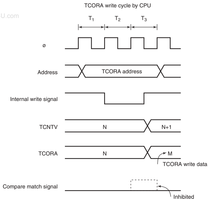
Figure 11.12 Contention between TCORA Write and Compare Match
