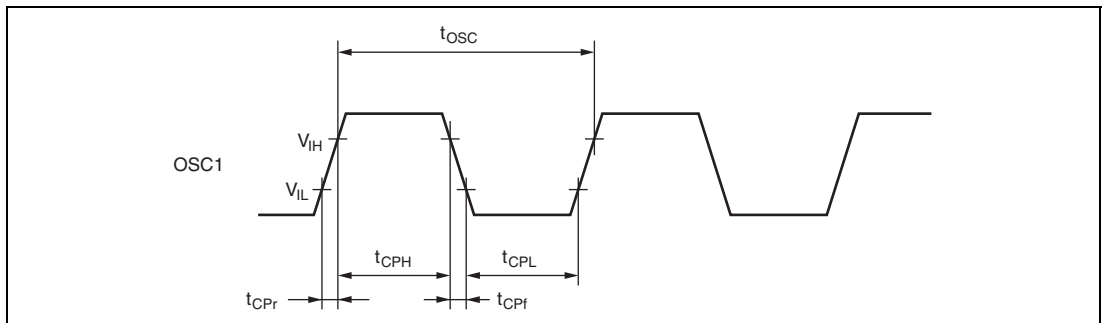
Figure 20.1 System Clock Input Timing www.DataSheet4U.com
