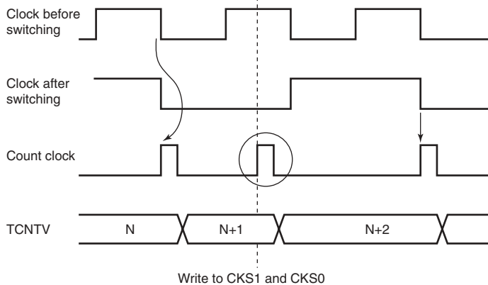
Figure 11.13 Internal Clock Switching and TCNTV Operation
