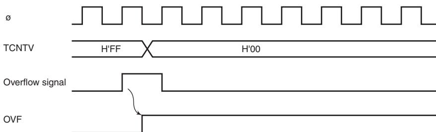
Figure 11.4 OVF Set Timing
