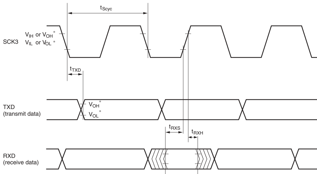
Figure 20.5 SCK3 Input Clock Timing
