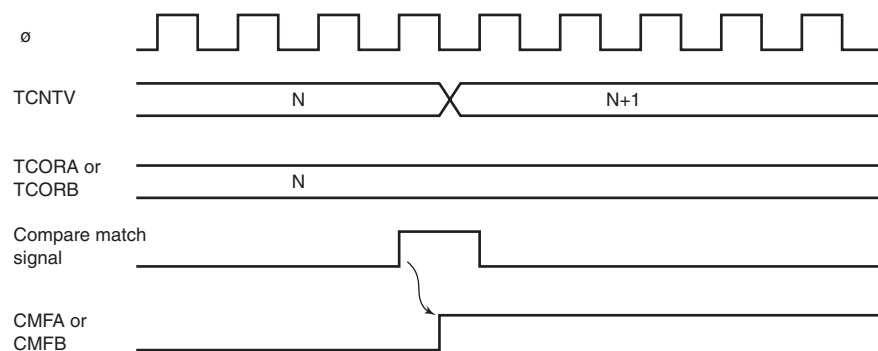
Figure 11.5 CMFA and CMFB Set Timing
