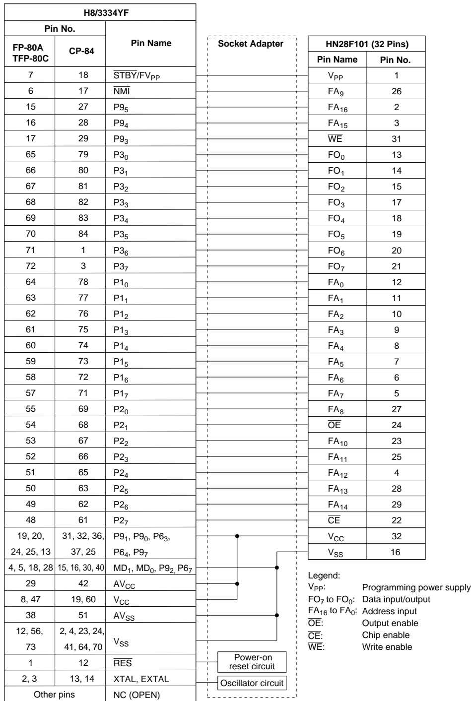
Figure 19.14 Wiring of Socket Adapter
