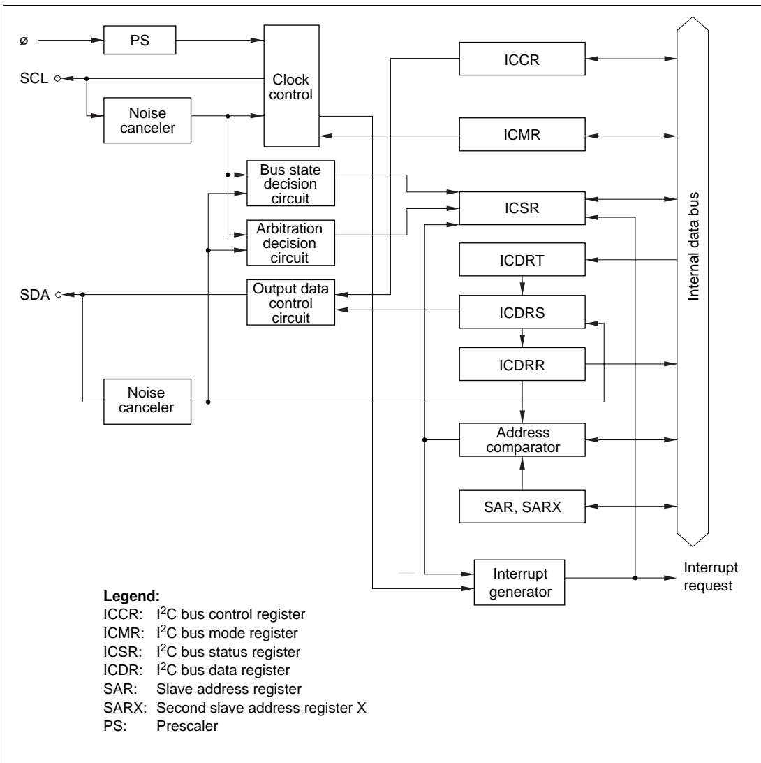
Figure 18-1 Block Diagram of I²C Bus Interface
