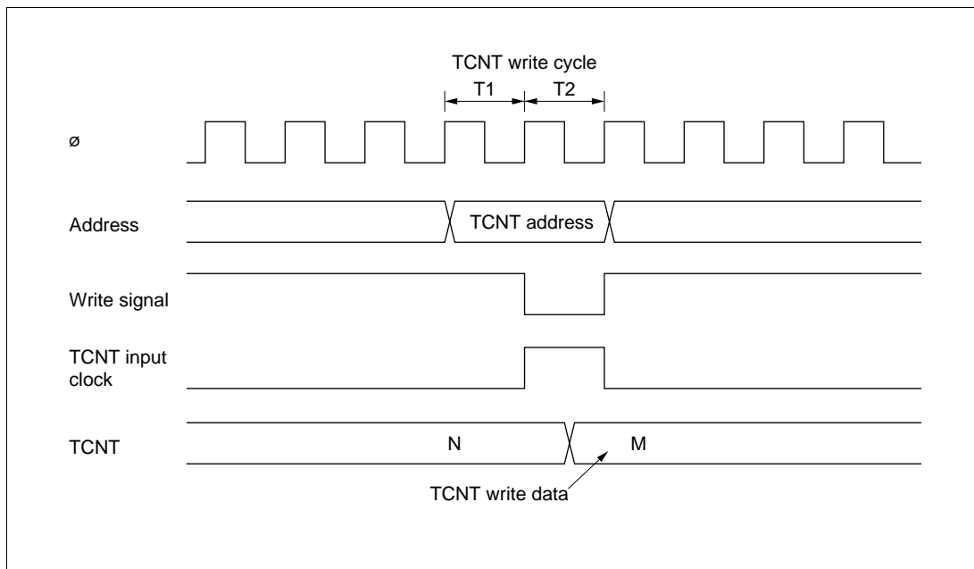
Figure 11-50 Contention between TCNT Write and Increment Operations
