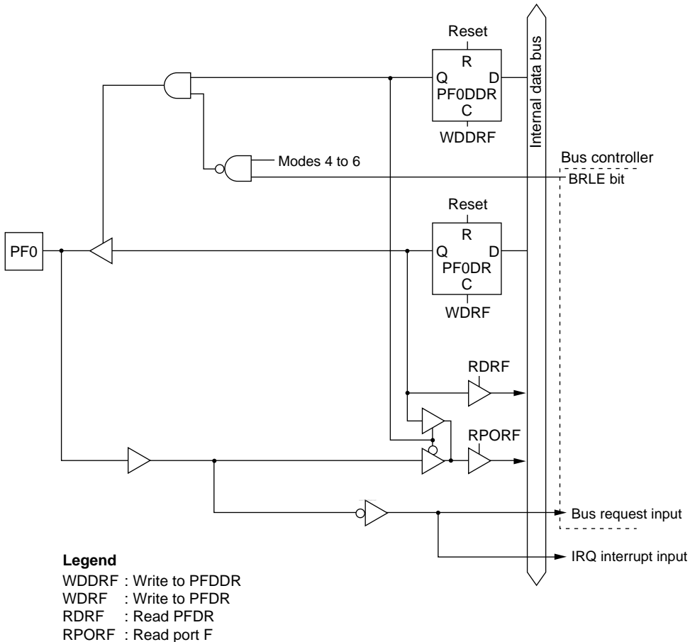
Figure C-11 (a) Port F Block Diagram (Pin PF0)
