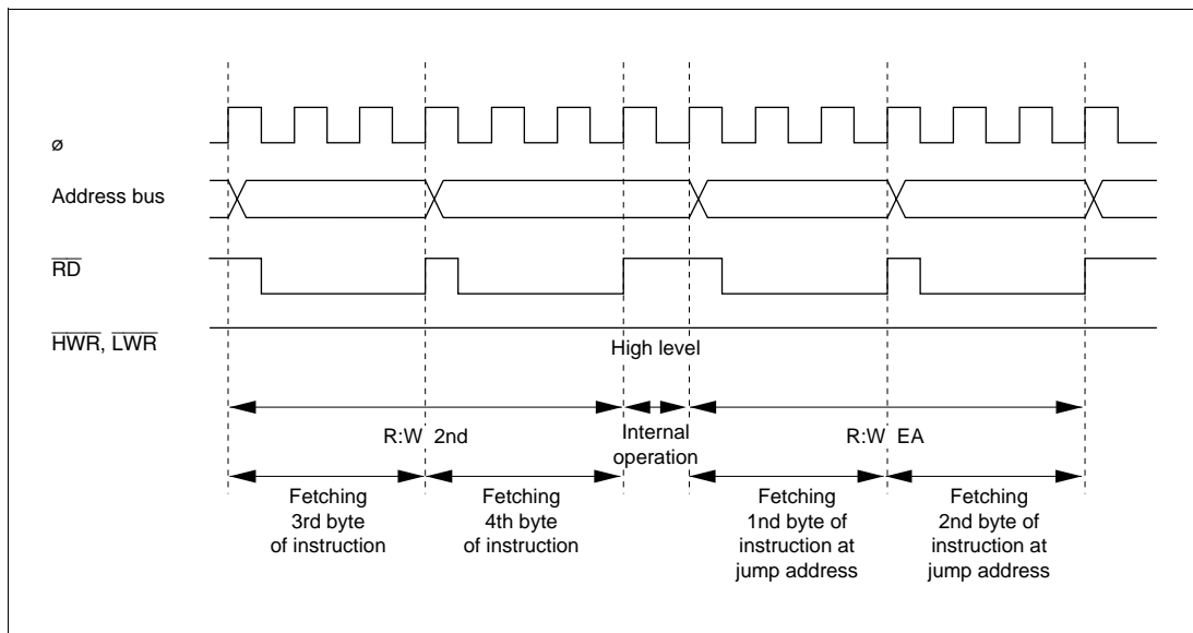
Figure A-1 Address Bus, \overline{\text{RD}} , \overline{\text{HWR}} , and \overline{\text{LWR}} Timing (8-Bit Bus, Three-State Access, No Wait States)
