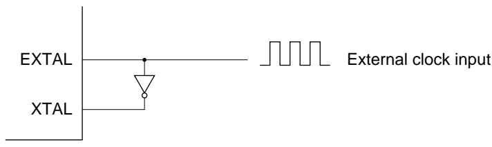
(b) Complementary clock input at XTAL pin
