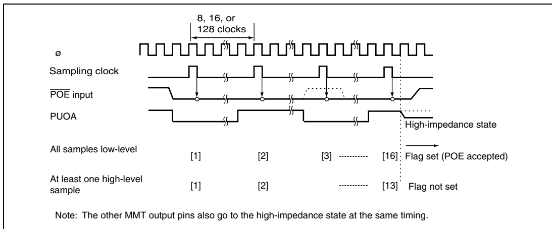
Figure 11-20 Low Level Detection Operation
