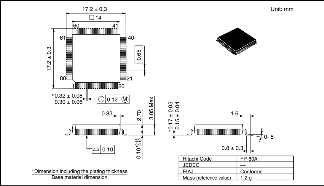
Figure D.1 FP-80A Package Dimensions
