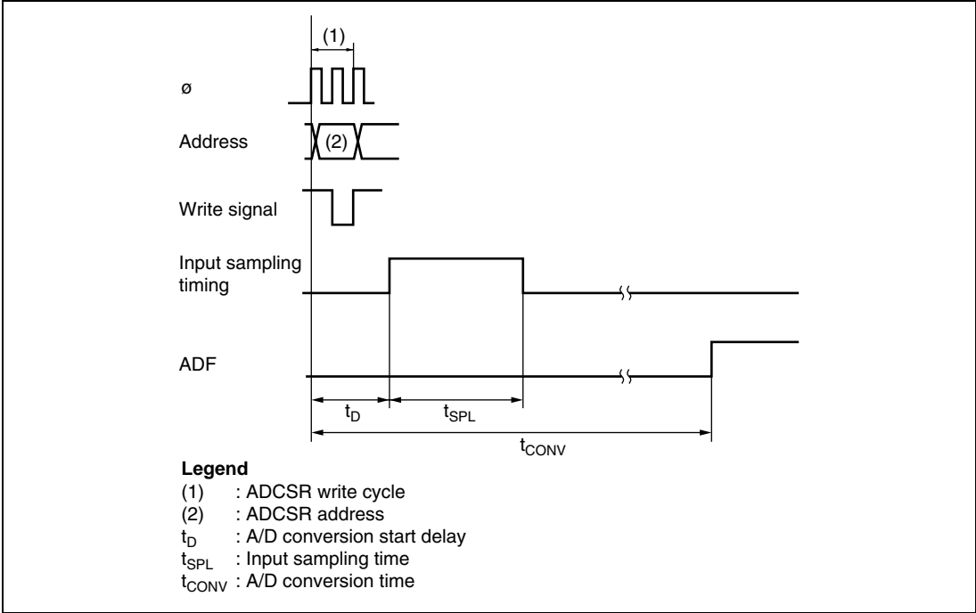
Figure 16-2 A/D Conversion Timing
