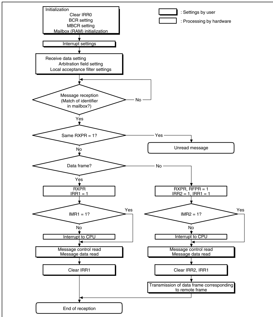
Figure 15-11 Reception Flowchart
