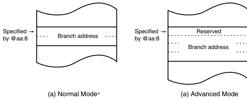
Figure 2-12 Branch Address Specification in Memory Indirect Mode
