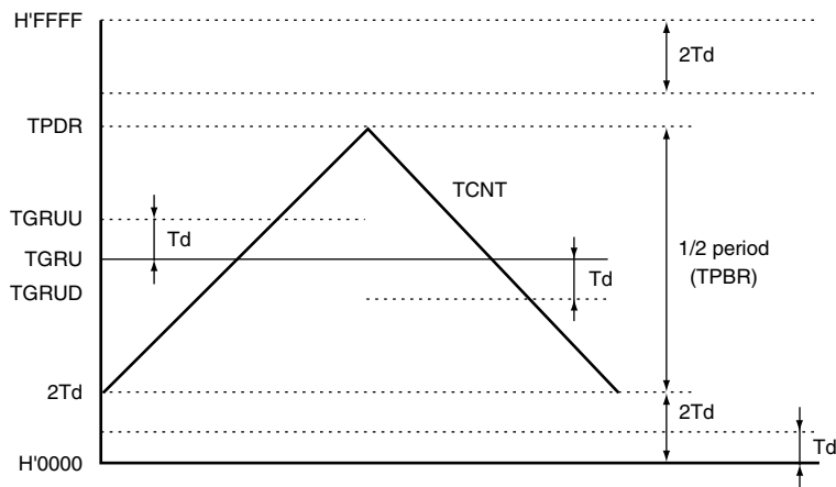
Figure 11-4 Example of TCNT Count Operation
