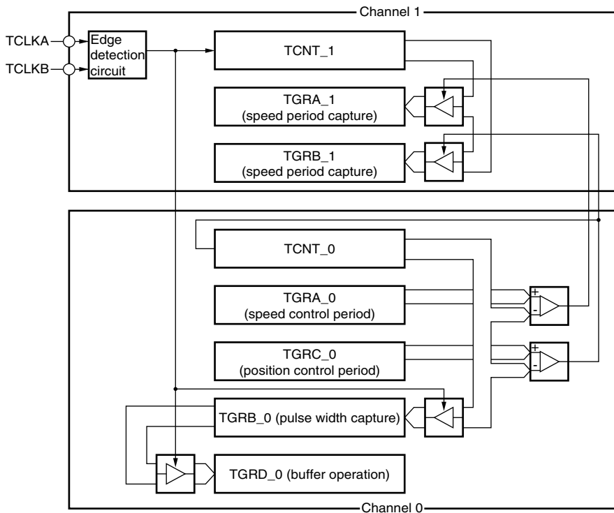
Figure 10-29 Phase Counting Mode Application Example
