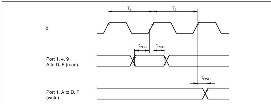
Figure 21-6 I/O Port Input/Output Timing
