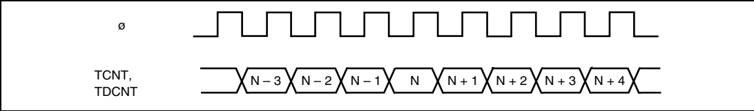
Figure 11-9 Count Timing
