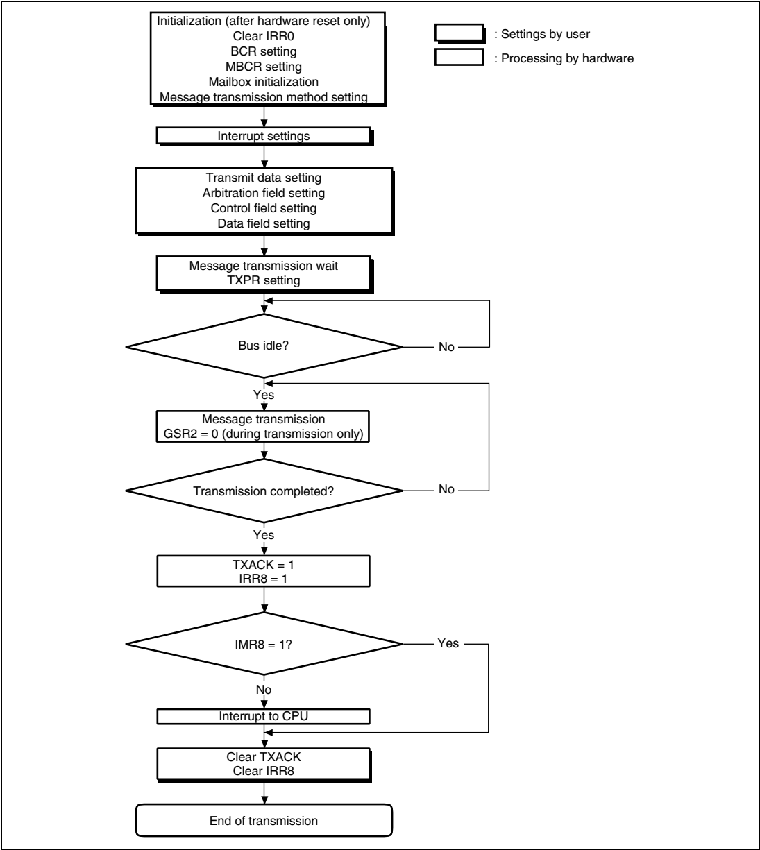
Figure 15-9 Transmission Flowchart
