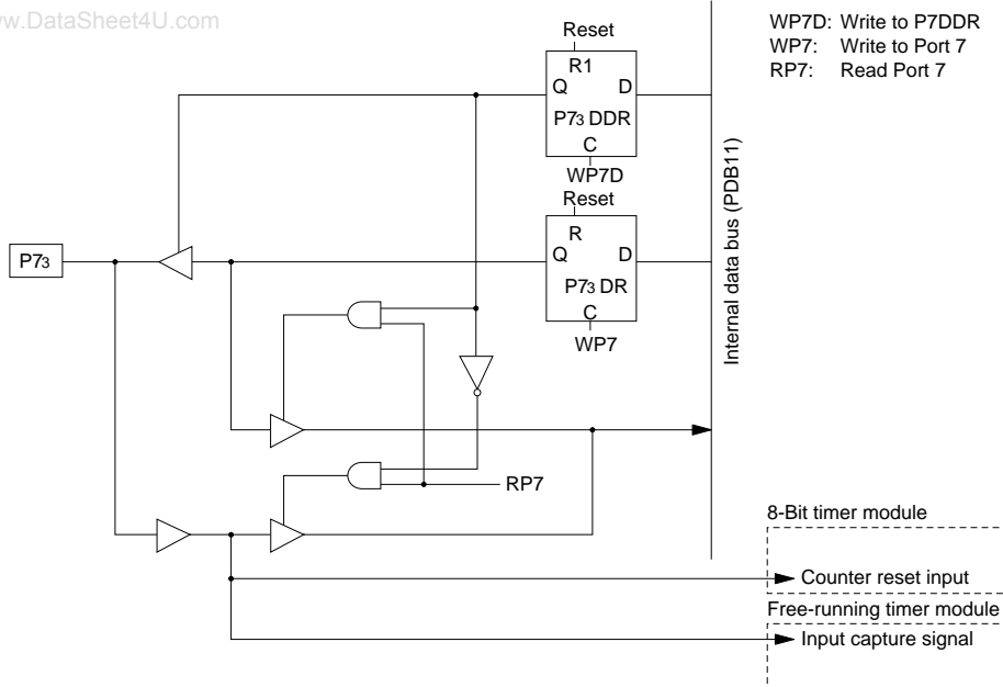
Figure C-7 (c) Schematic Diagram of Port 7, Pin P73
