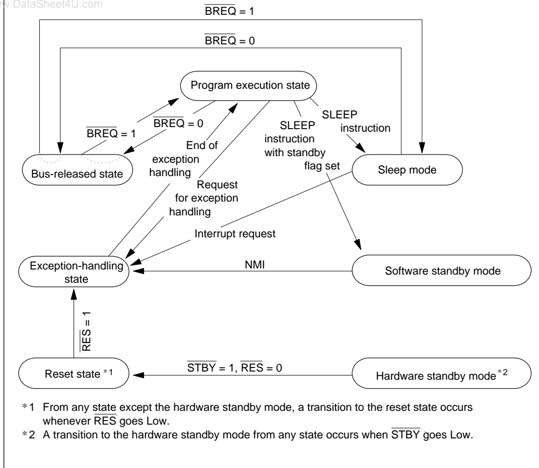
Figure 3-12 State Transitions
