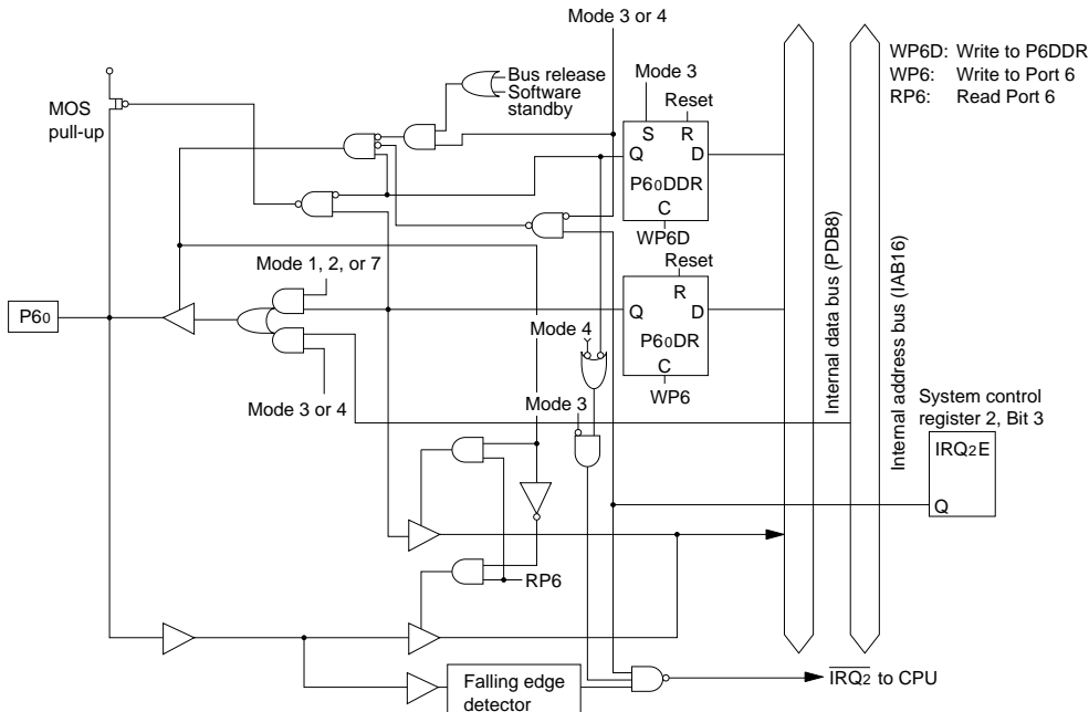
Figure C-6 (a) Schematic Diagram of Port 6, Pin P60
