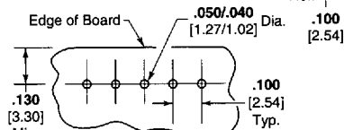
Recommended Mounting Hole Size for .062 [1.57] Thk. PC Board
