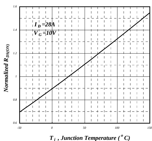
Fig 4. Normalized On-Resistance
