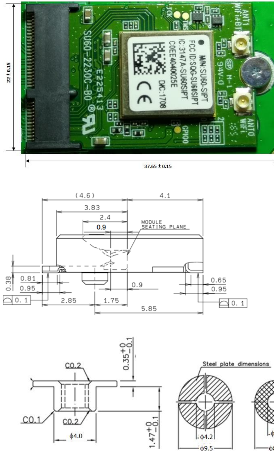
Figure 9: Mounting information of the 60-2230C and recommended layout pattern for the stand-off
