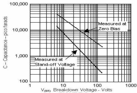
FIGURE 3 Typical Capacitance vs Breakdown Voltage
