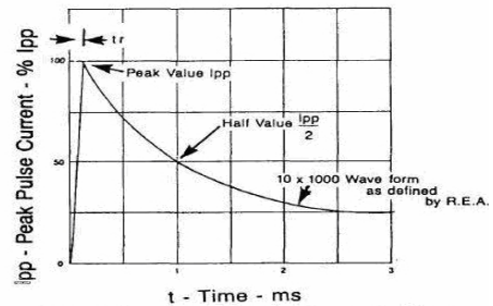
Test waveform parameters: t_r = 10 \mu s , t_p = 1000 \mu s FIGURE 2 Pulse Waveform
