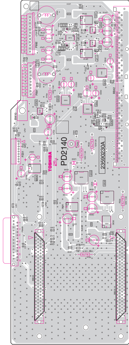
MOTHER BOARD PD2140B (U102) TOP (COMPONENT) SIDE
