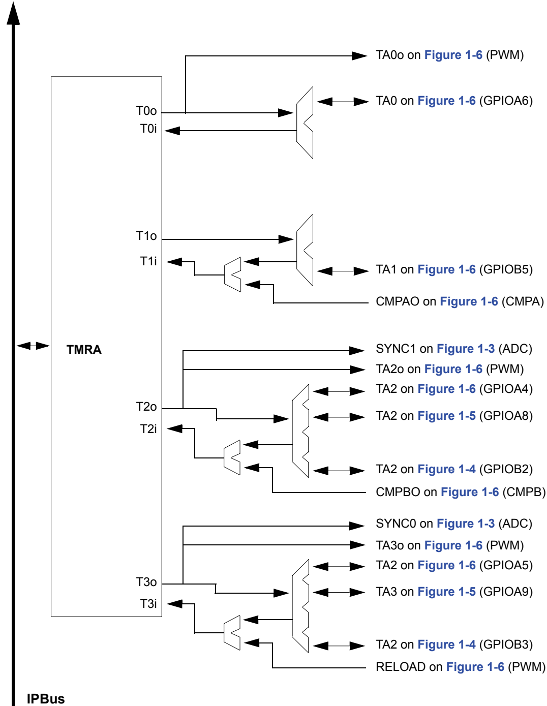
Figure 1-7 56F8036 I/O Pin-Out Muxing (Part 5/5)
