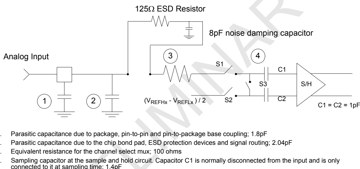
Figure 10-18 Equivalent Circuit for A/D Loading
