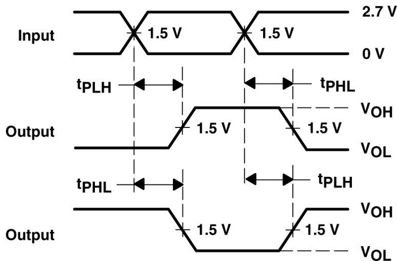
FIGURE 4. PROPAGATION DELAY TIMES INVERTING AND NON-INVERTING OUTPUTS
