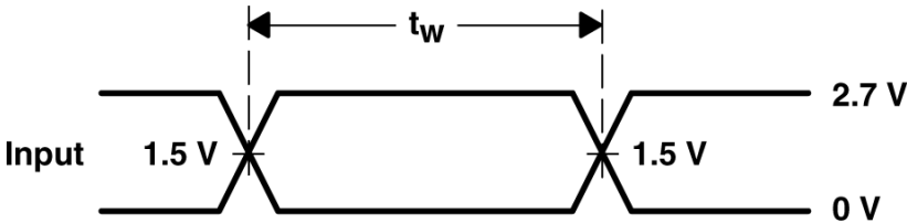
FIGURE 2. PULSE DURATION
