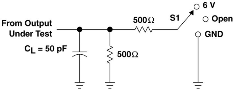
FIGURE 1. LOAD CIRCUIT
