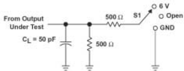
FIGURE 1. LOAD CIRCUIT
