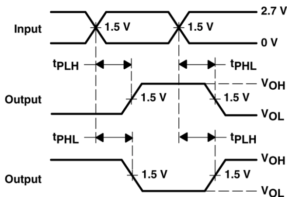
FIGURE 4. PROPAGATION DELAY TIMES INVERTING AND NONINVERTING OUTPUTS
