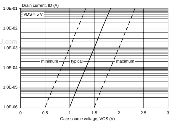
Fig.11. Sub-threshold drain current.
