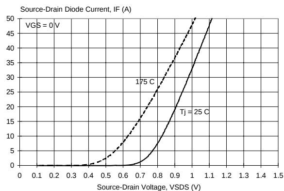
Fig.14. Typical reverse diode current.
