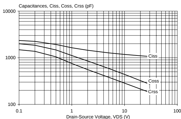
Fig.12. Typical capacitances, C_{iss} , C_{oss} , C_{rss} .
