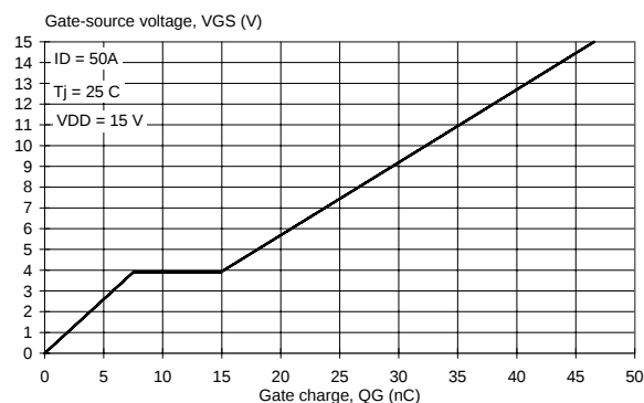
Fig.13. Typical turn-on gate-charge characteristics.
