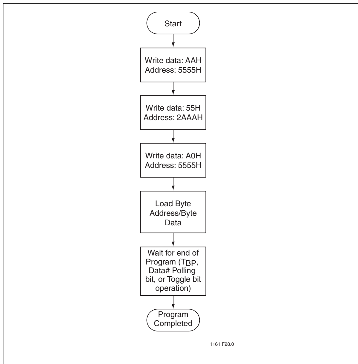
Figure 25: Byte-Program Algorithm
